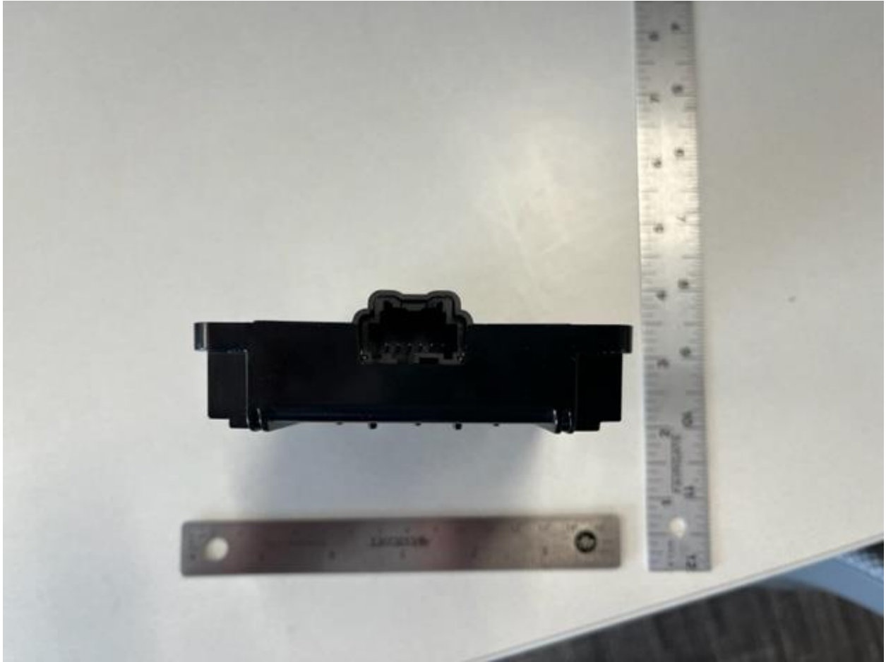
Figure 3 4200 Connector View
