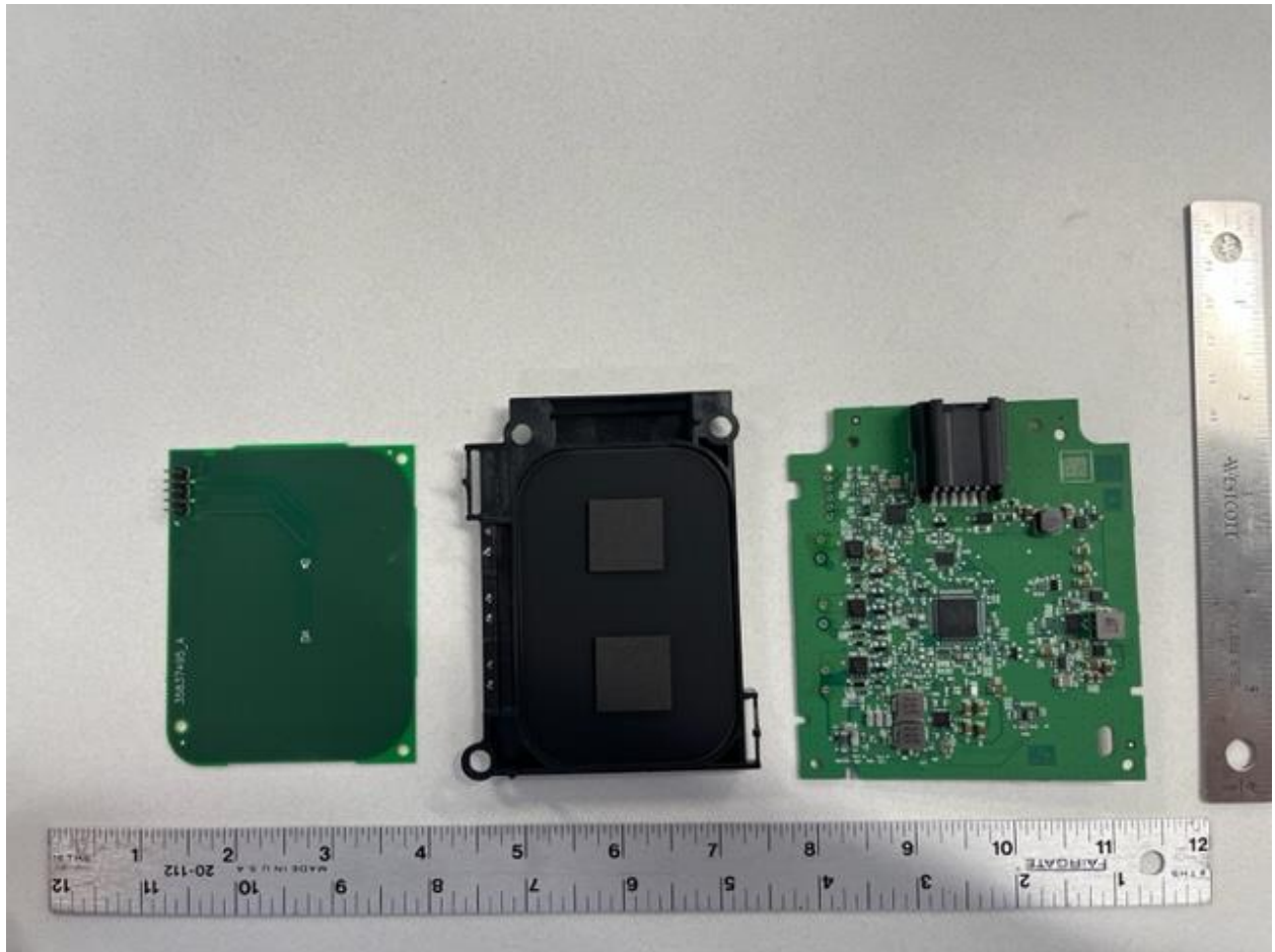
Figure 3 4200 PCBs Top
