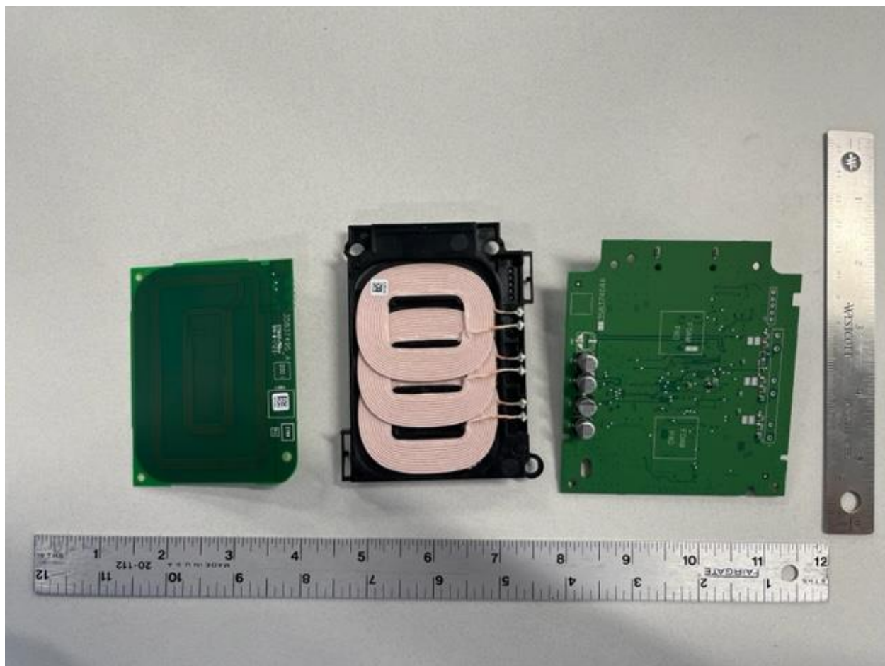
Figure 4 4200 PCBs Bottom
