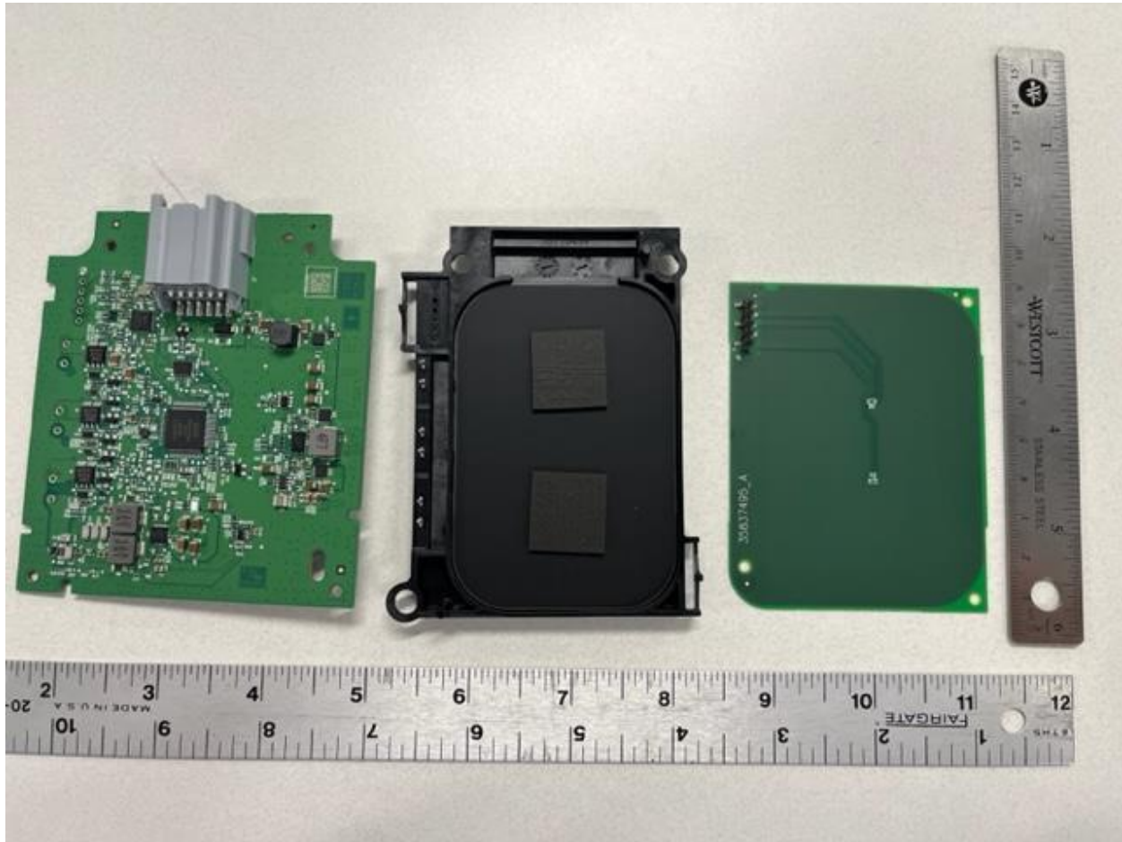
Figure 1 4199 PCBs Top
