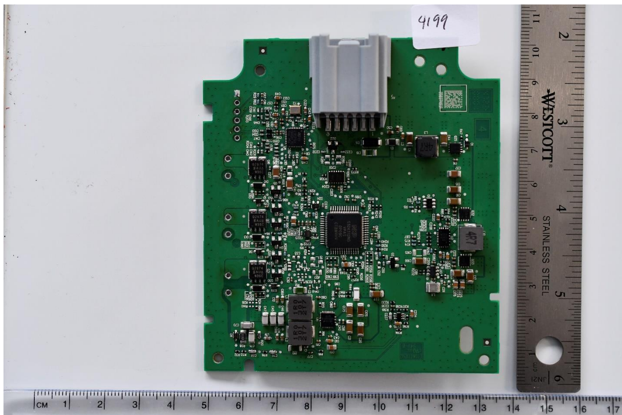
Figure 3 PCB side 1
