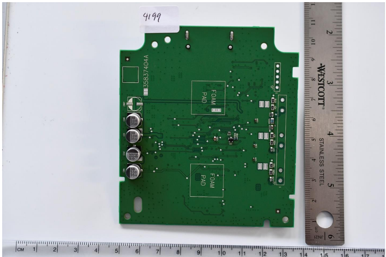
Figure 4 PCB side 2
