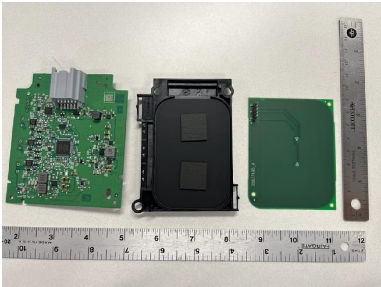
Figure 3 4199 PCBs Top
