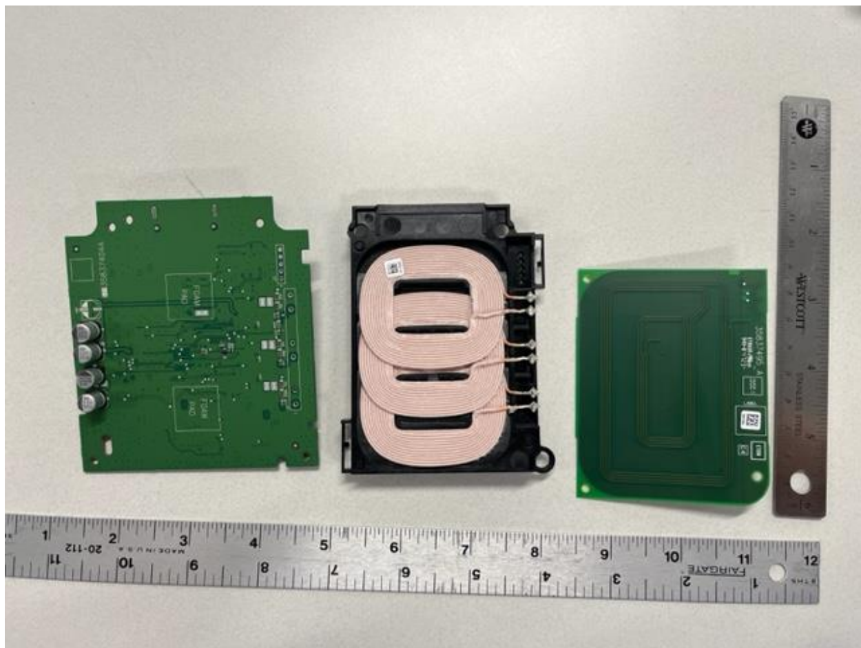
Figure 4 4199 PCBs Bottom
