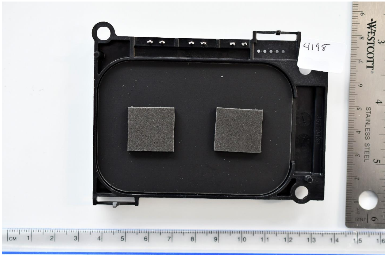
Figure 6 Coil Board side 2
