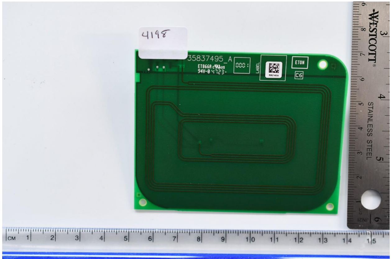
Figure 7 Antenna Board side 1
