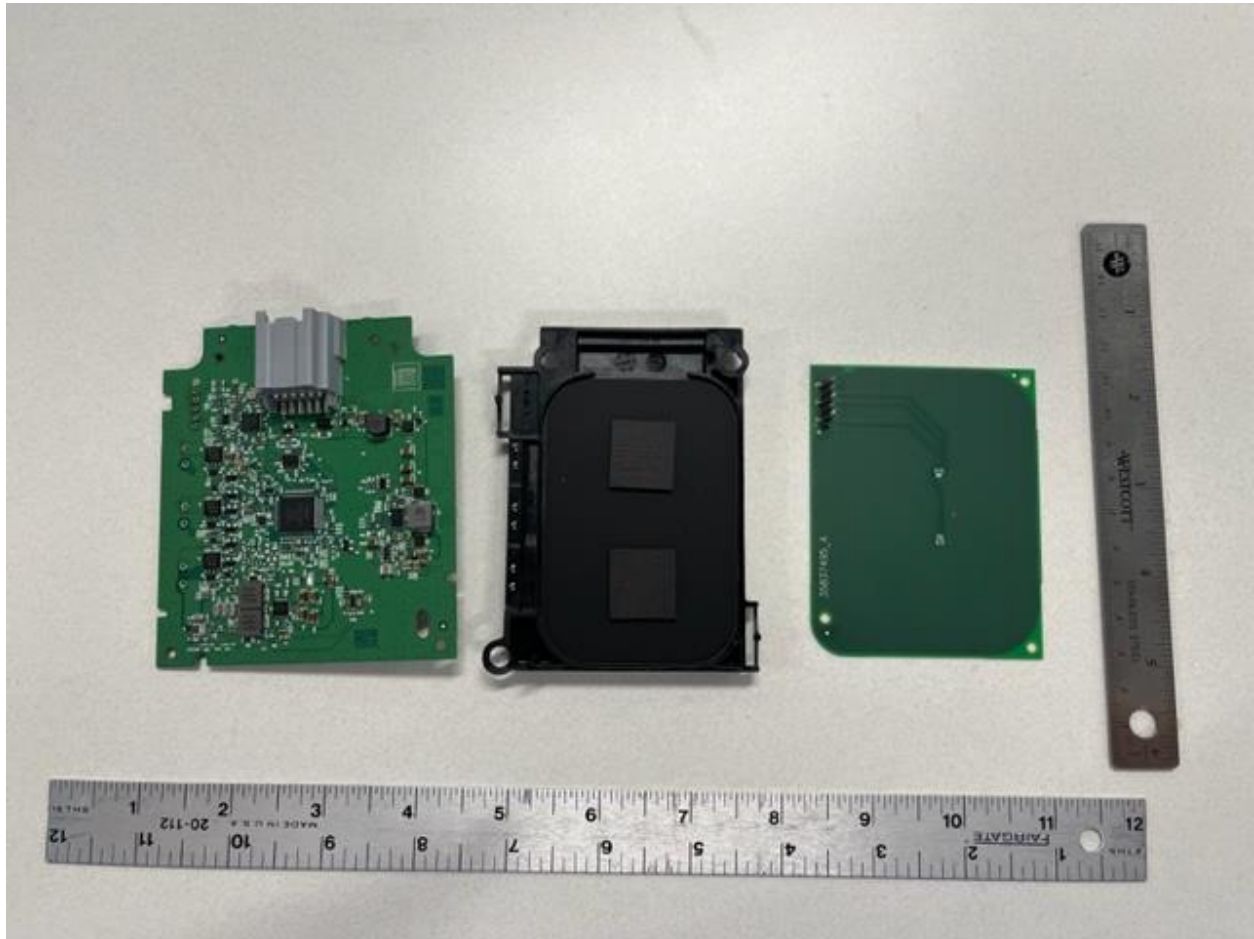
Figure 1 4198 PCBs Top
