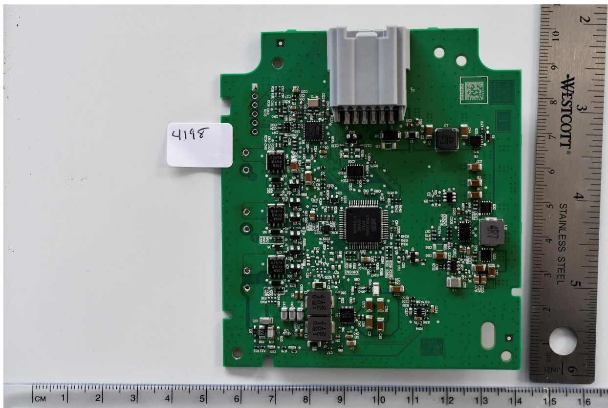
Figure 6 PCB side 1
