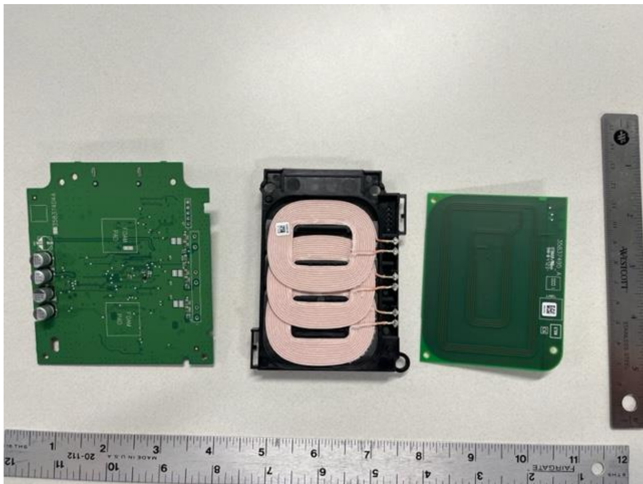
Figure 4 4198 PCBs Bottom
