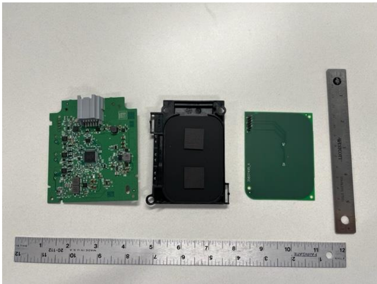
Figure 3 4198 PCBs Top
