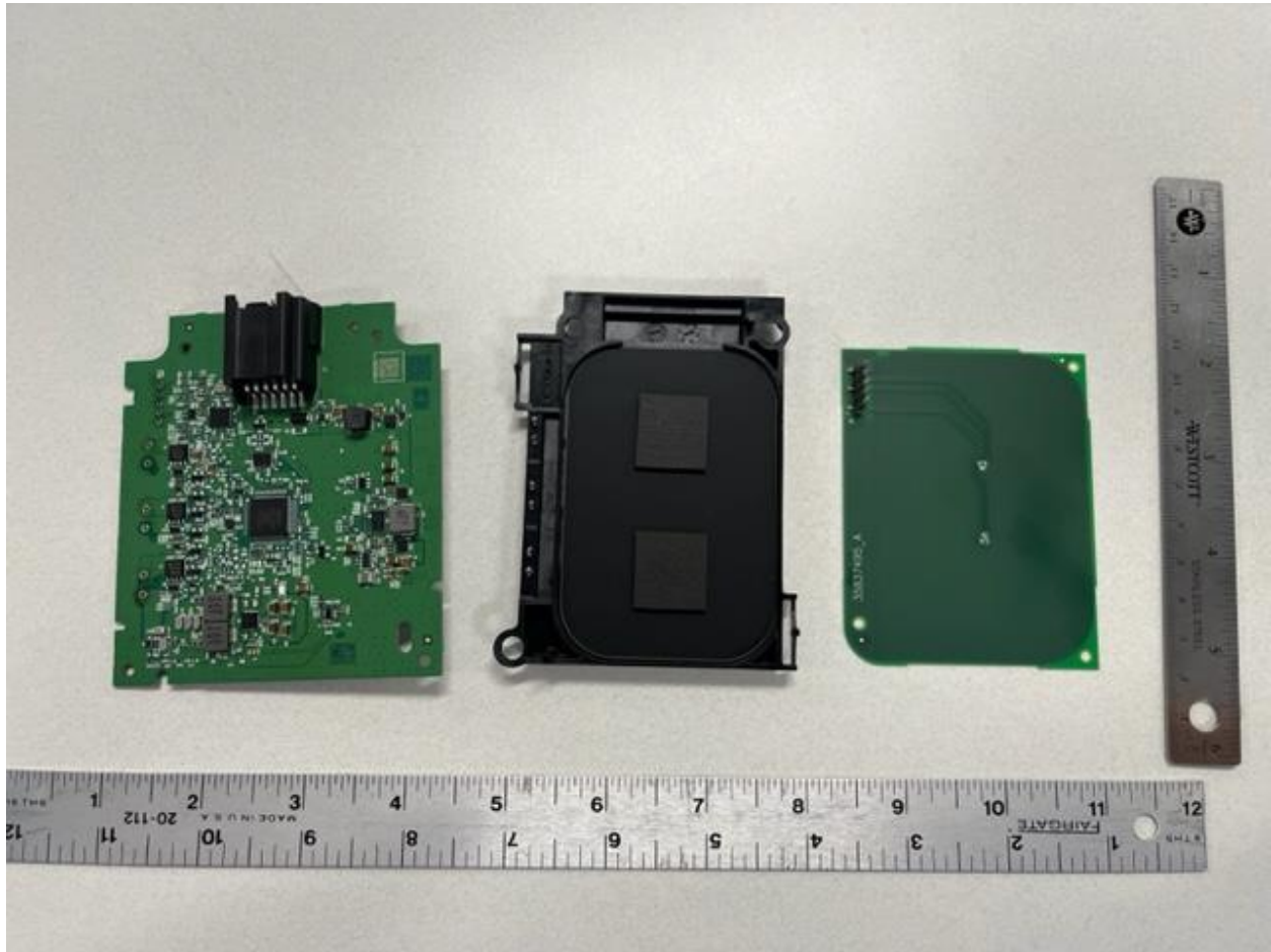
Figure 1 4197 PCBs Top
