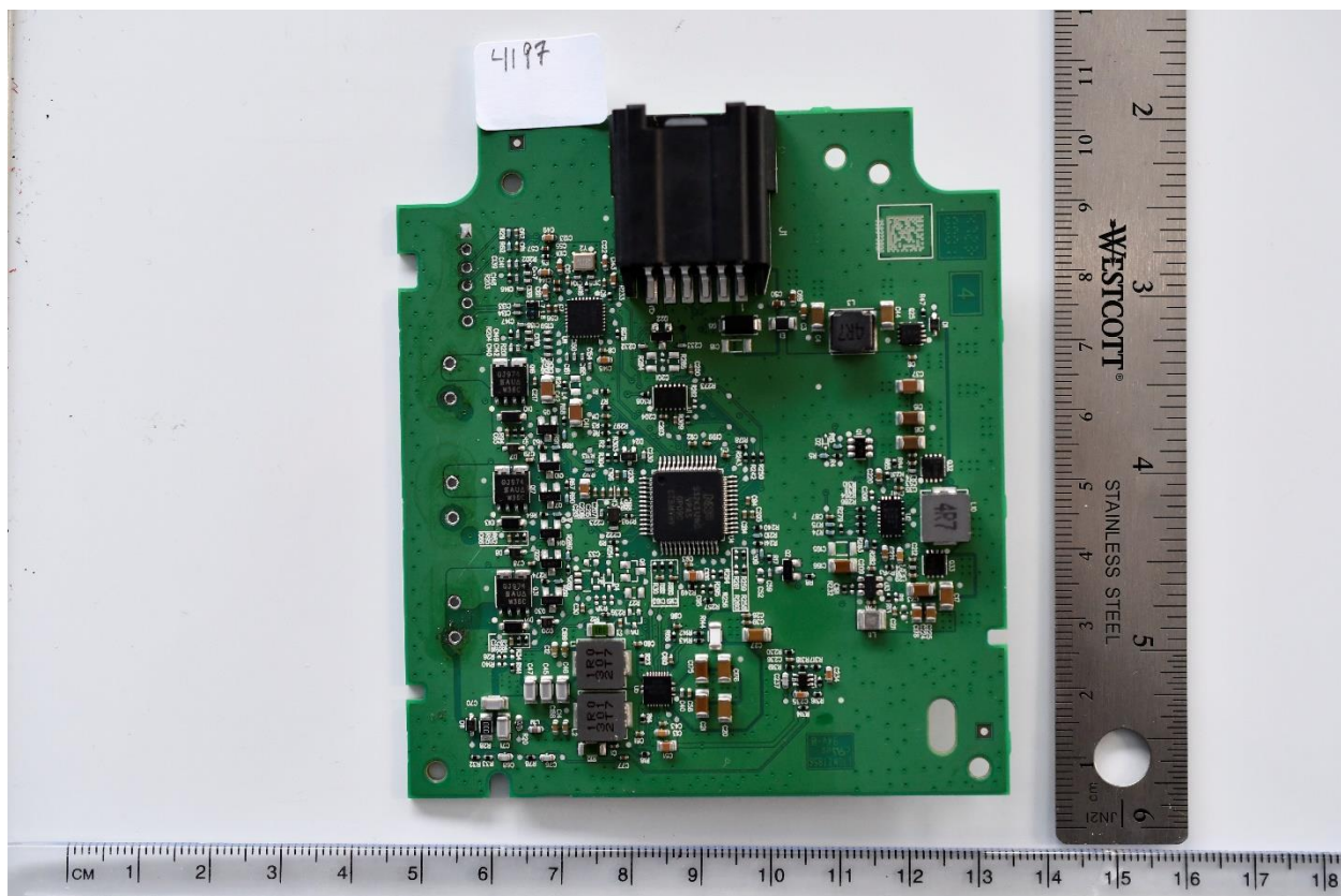
Figure 6 PCB side 1
