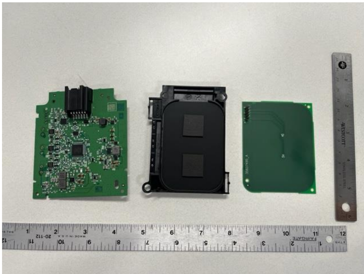
Figure 3 4197 PCBs Top
