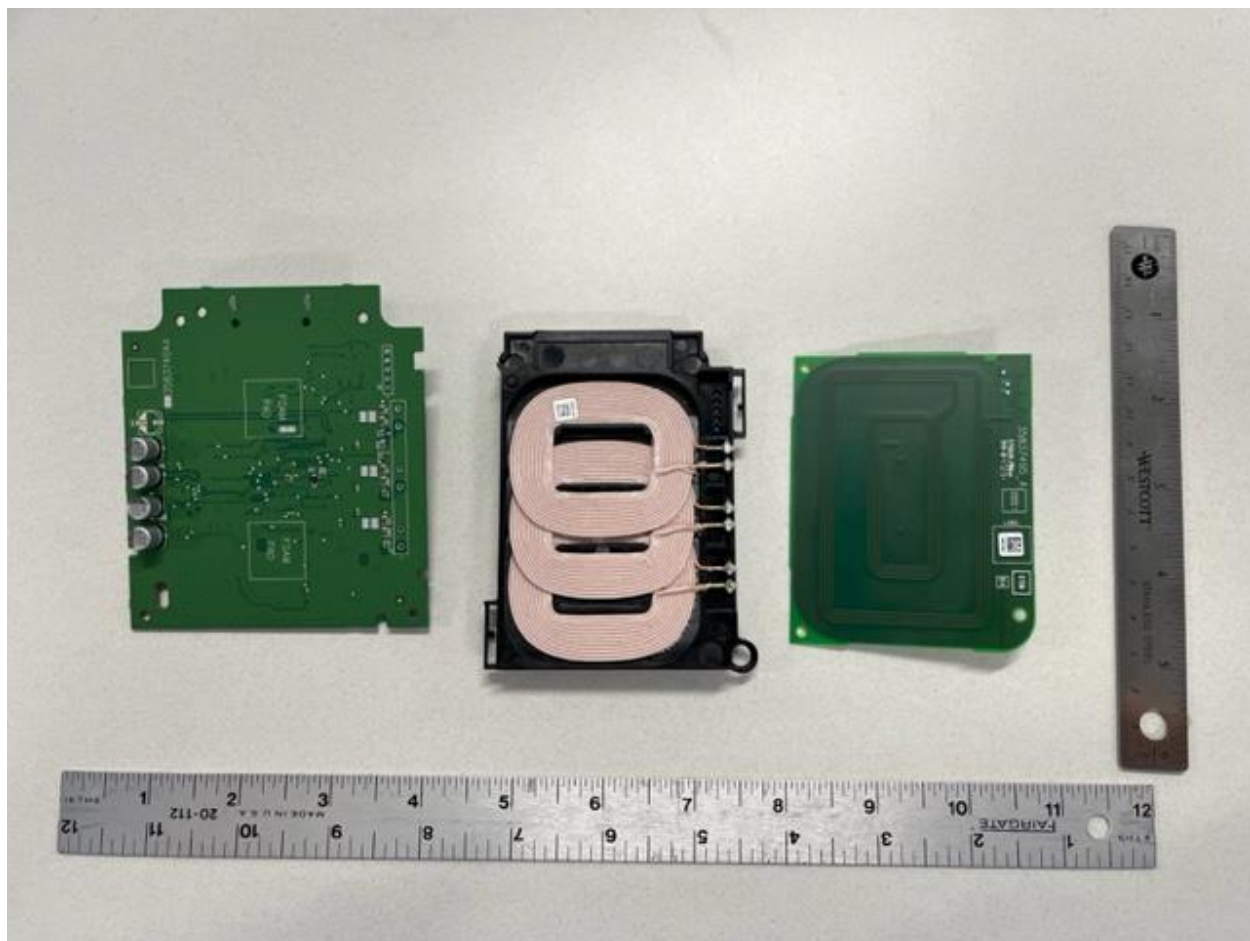
Figure 4 4197 PCBs Bottom
