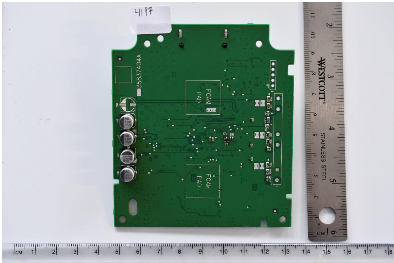
Figure 7 PCB side 2
