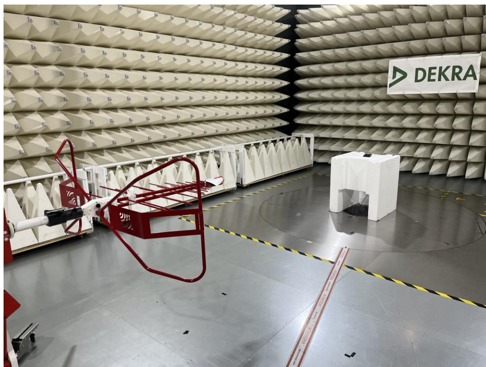
Figure B.6: Radiated Test setup 2
