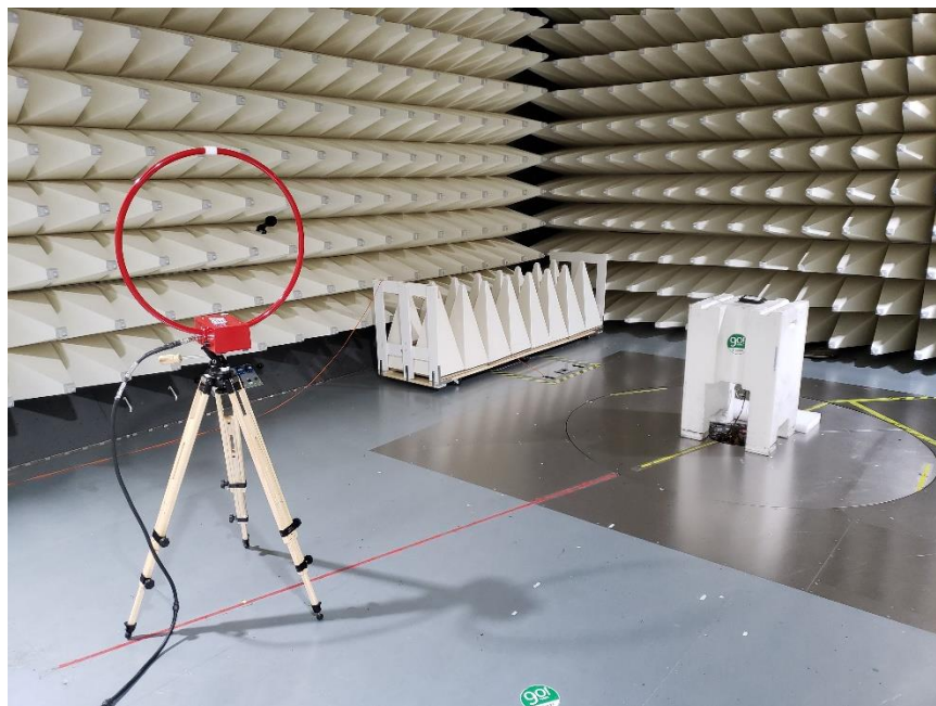
Figure B.5: Radiated Test setup 1
