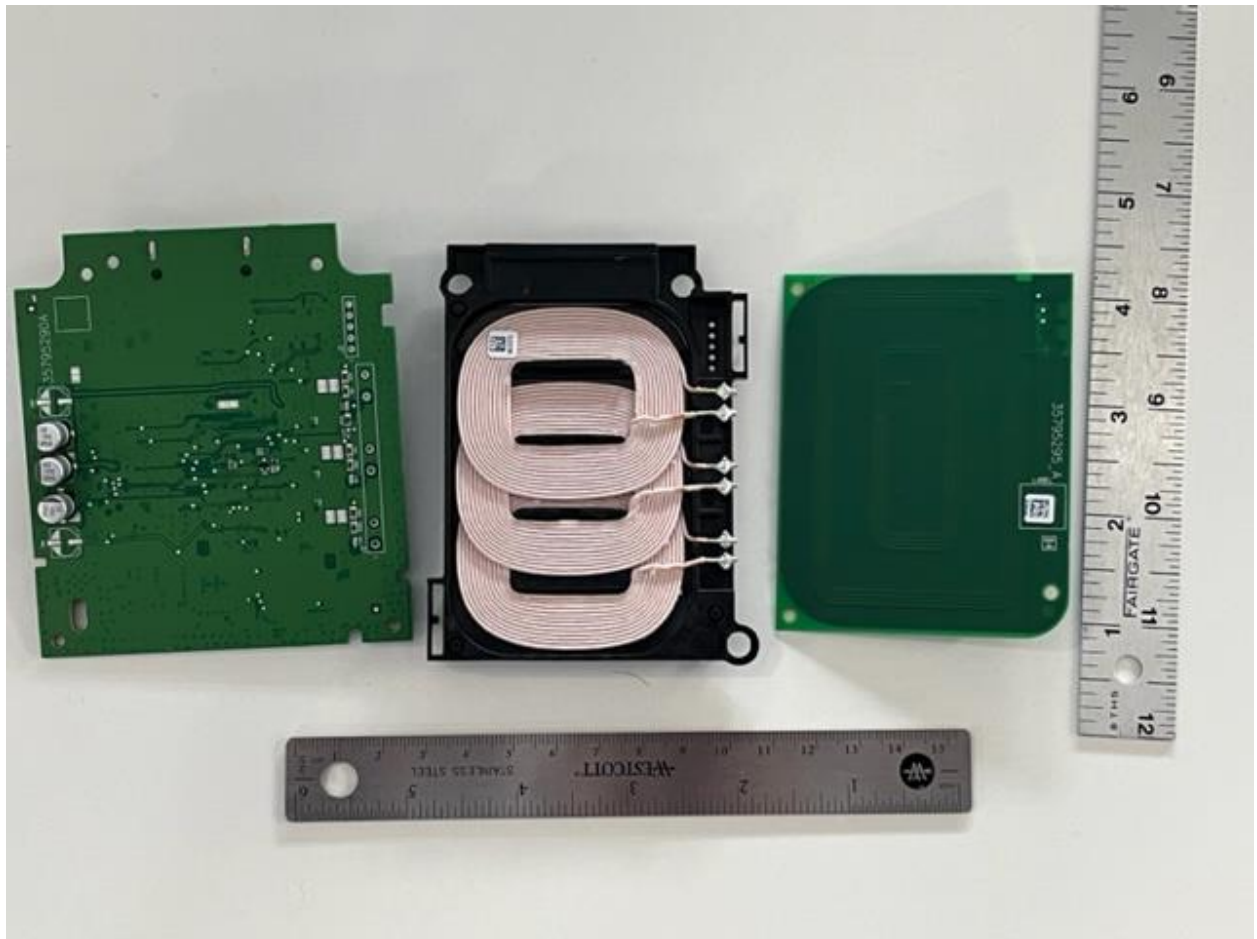
Figure 4 0621 PCBs Bottom
