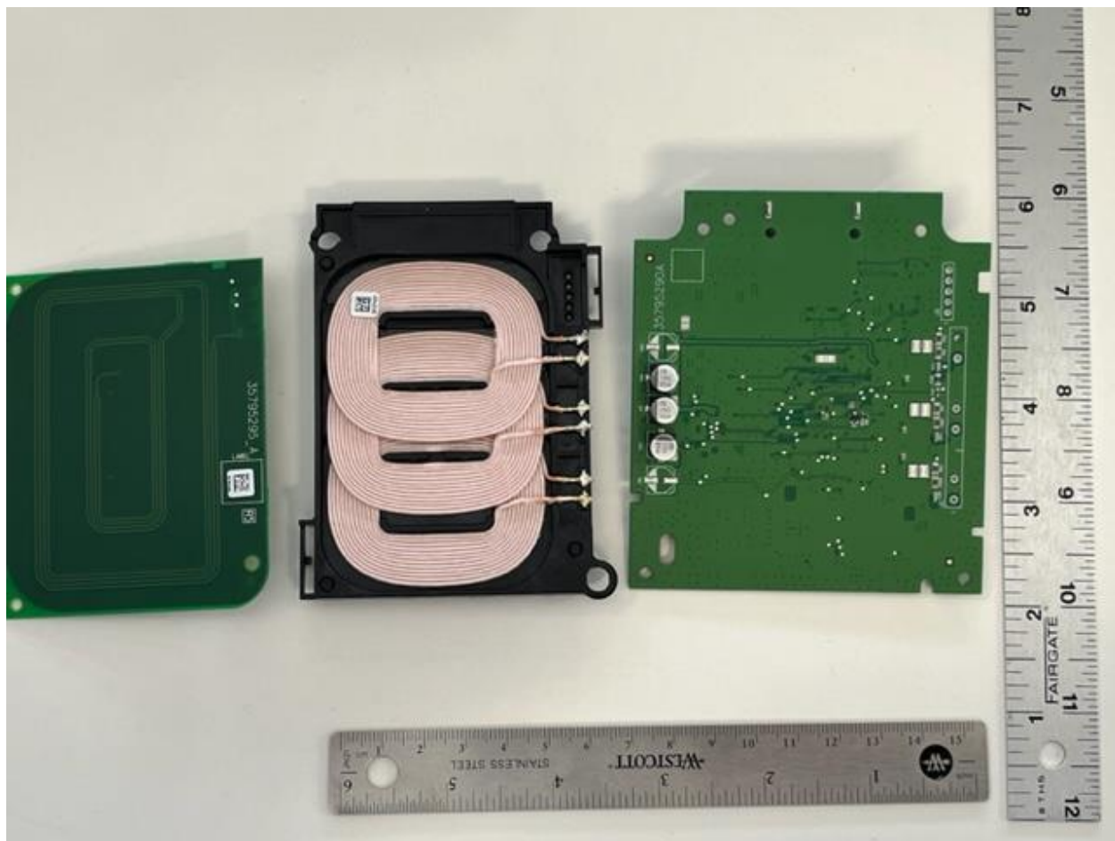
Figure 4 0618 PCBs Bottom
