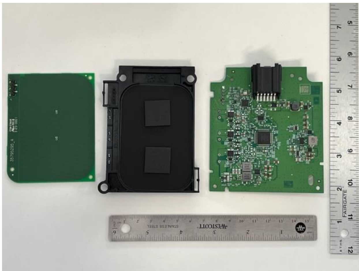
Figure 3 0618 PCBs Top
