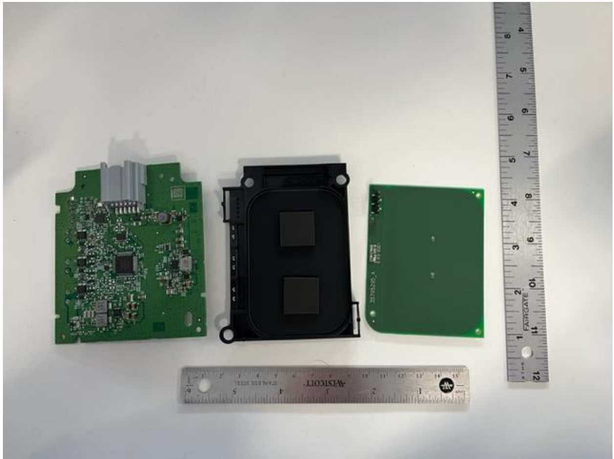
Figure 3 0620 PCBs Top
