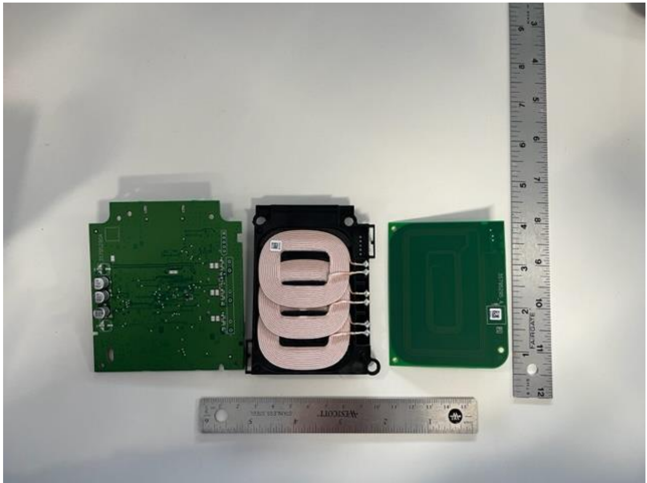
Figure 4 0620 PCBs Bottom
