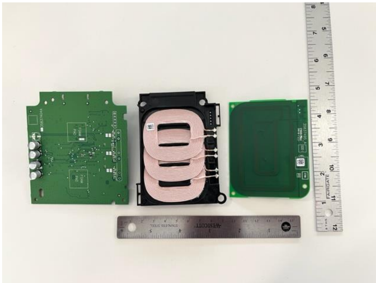
Figure 4 0619 PCBs Bottom
