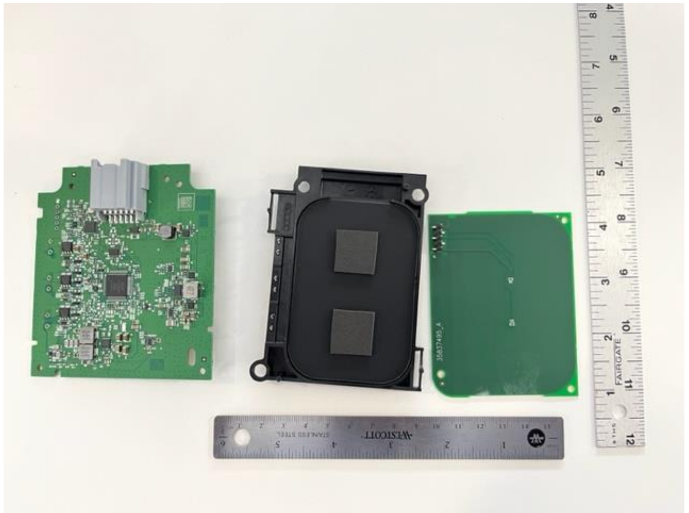
Figure 3 0619 PCBs Top
