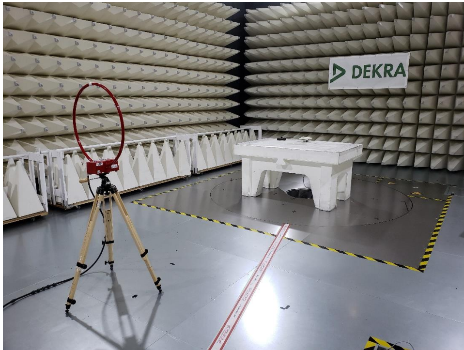
7. Low Range Radiated Emission test setup 9KHz to 30MHz
