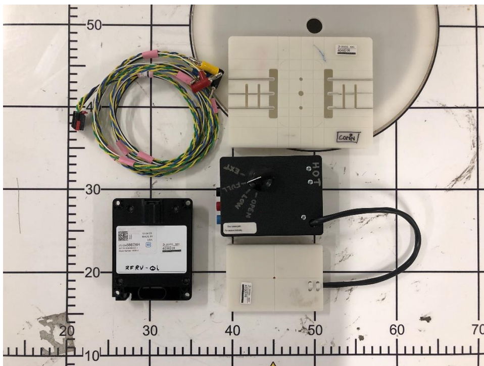
6. View of the DUT and accessories
