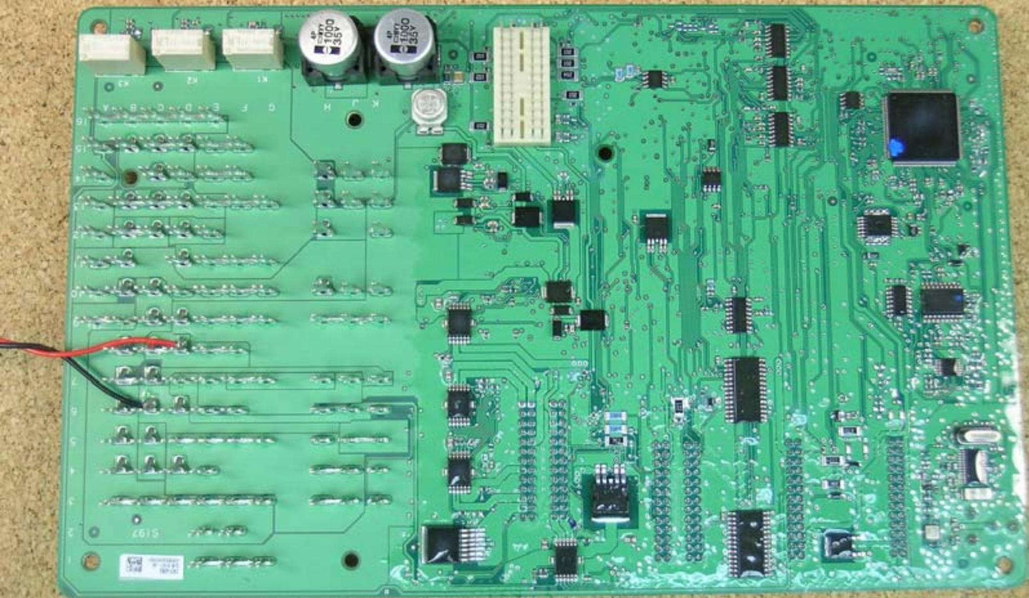
S197-06 PCB (bottom)
