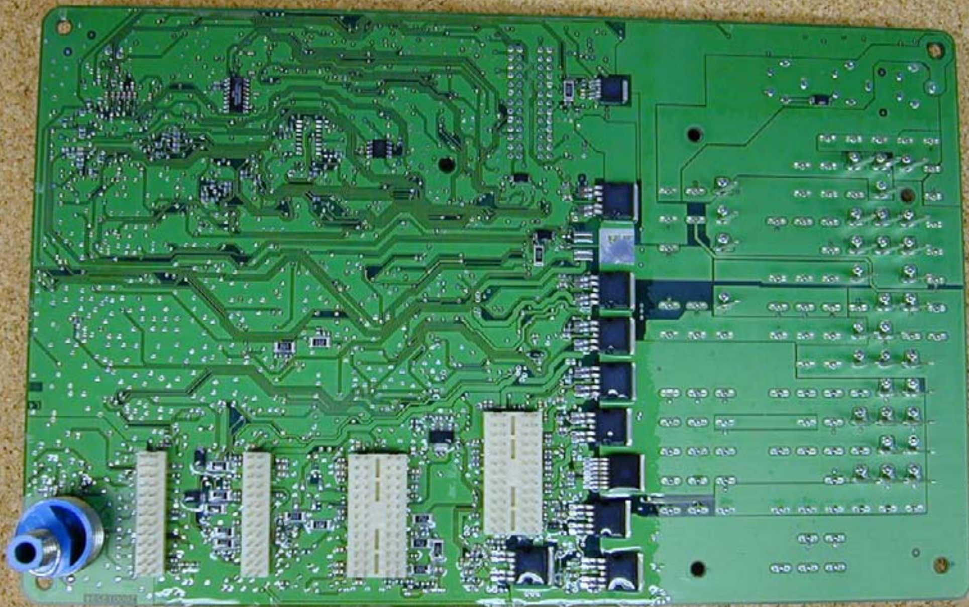
S197 PCB (bottom)
