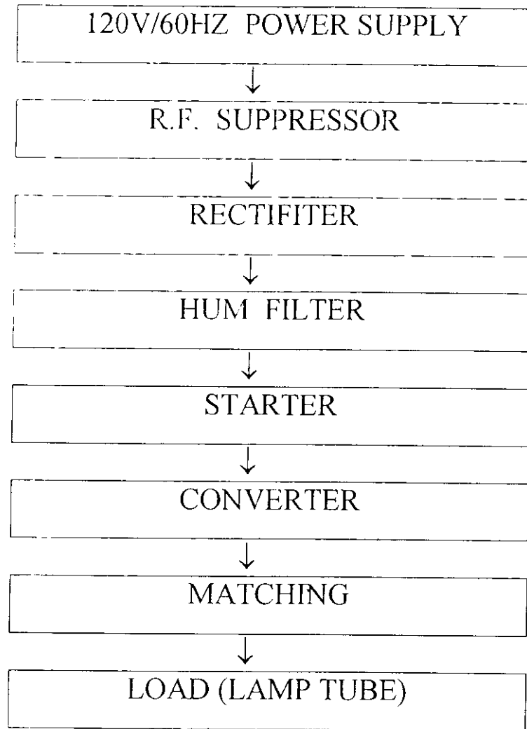
BLOCK DIAGRAM OF 120V DIRECT RECTIFYING LAMP SERIES
