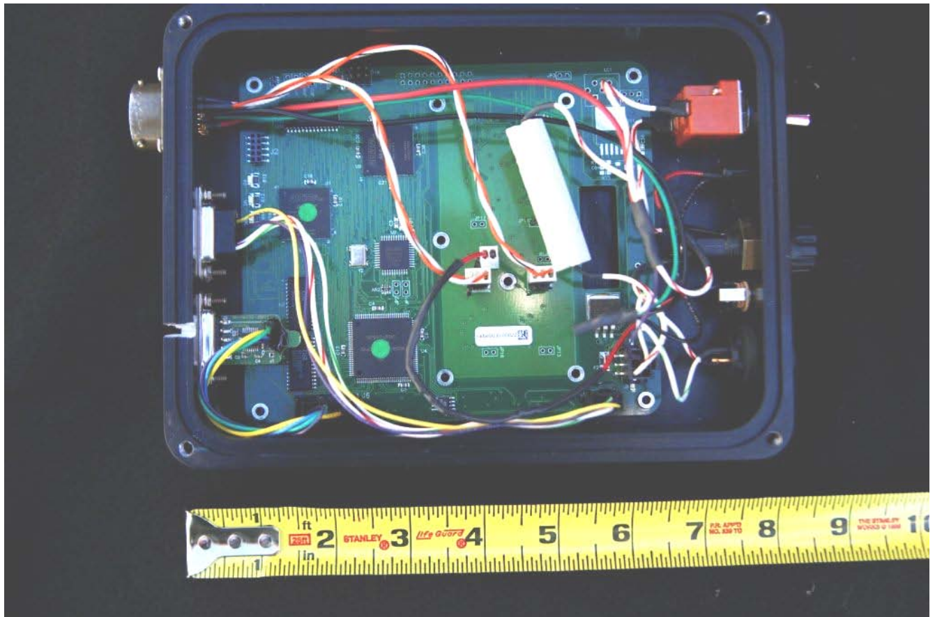
SC300 Radar Control Unit – Processor PCB Installed
