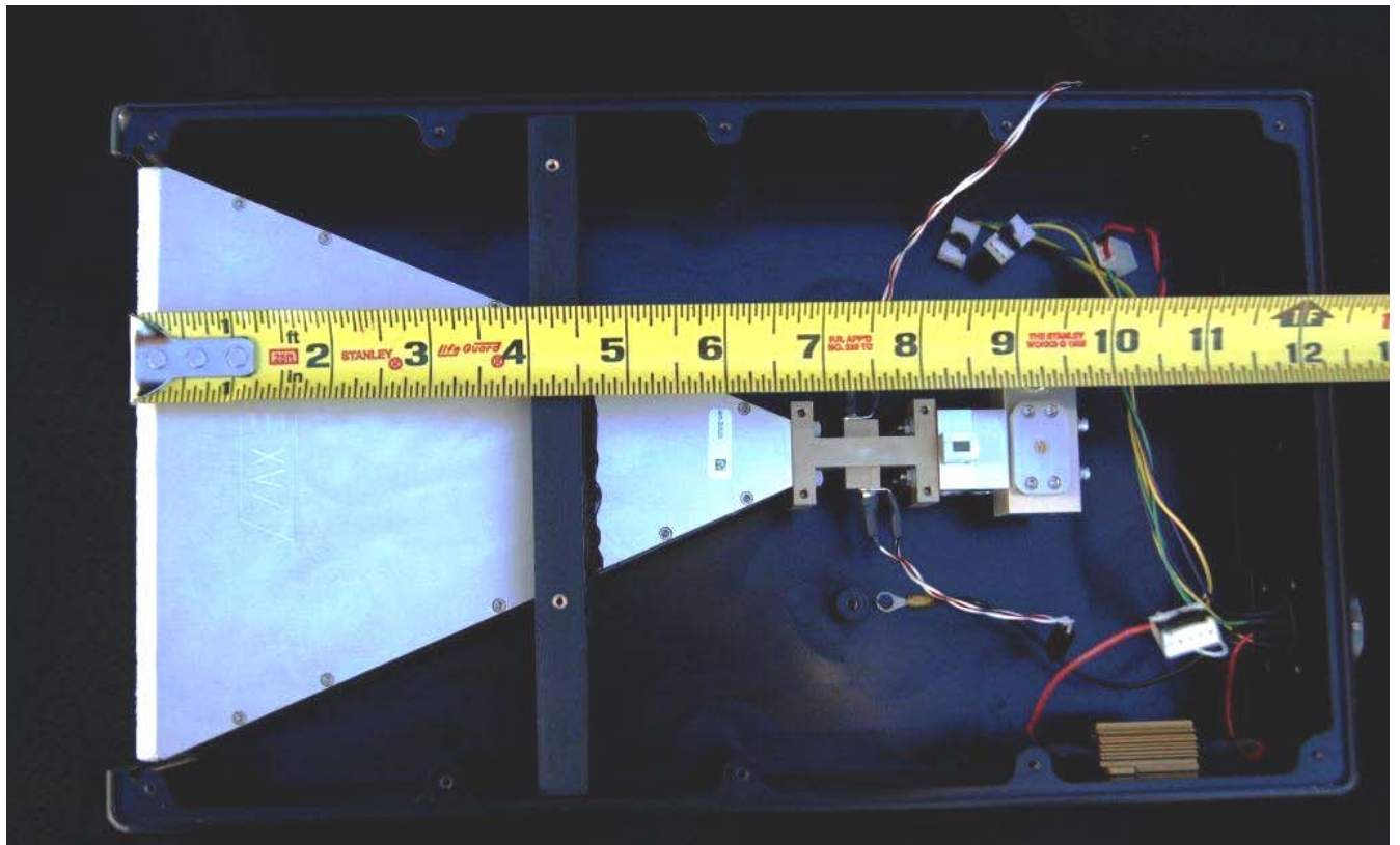
SC300 MICROWAVE ASSEMBLY
