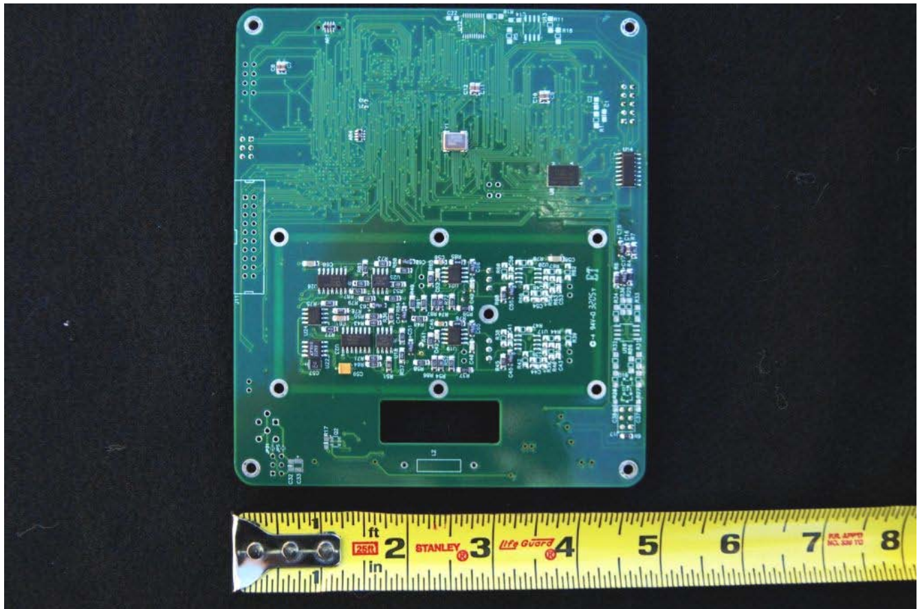
Radar Control Unit – PCB Bottom
