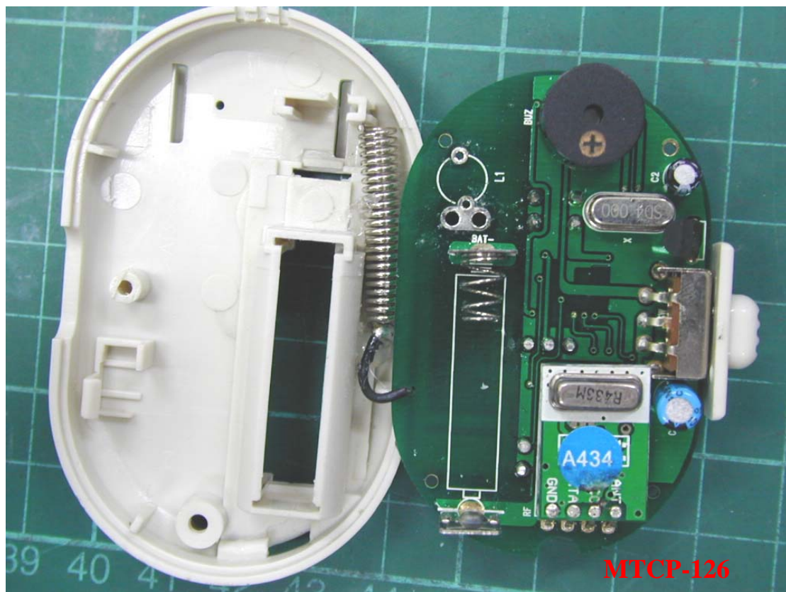
Photo 3: Internal photo of EUT (Transmitter)
