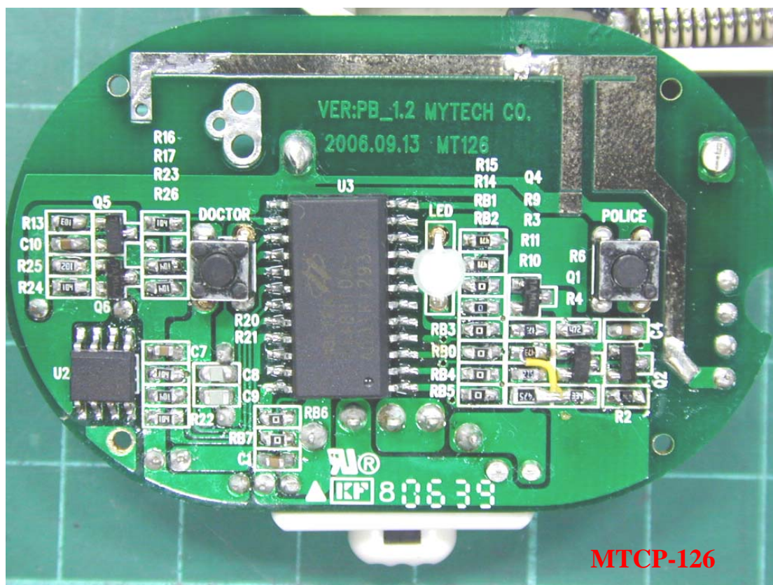
Photo 4: Internal photo of EUT (Transmitter)
