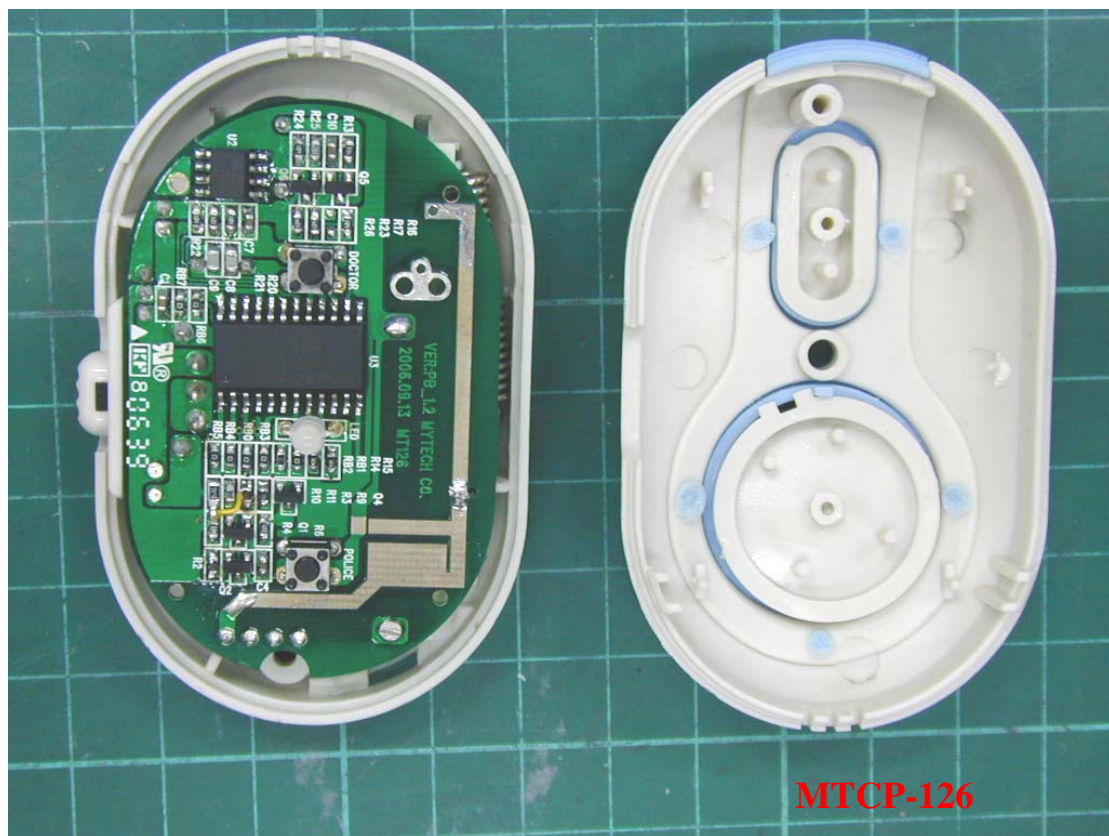
Photo 1: Internal photo of EUT (Transmitter)
