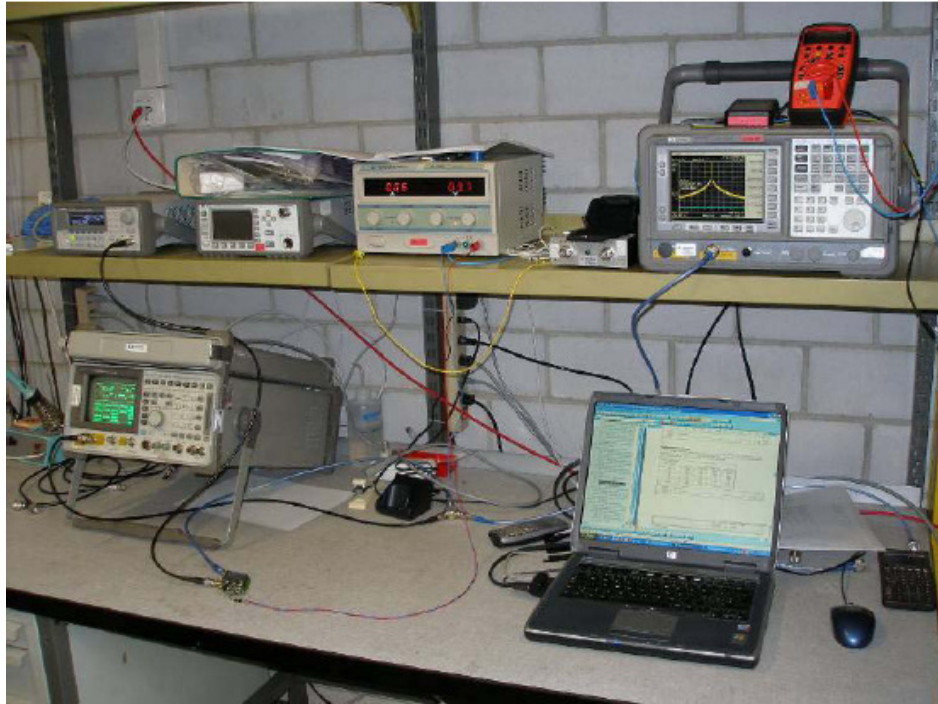
Fig 2 Modulation characteristics and occupied bandwidth
