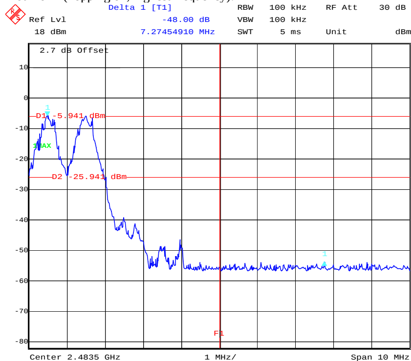
Plot 1 of 4 (hopping on, highest frequency):
