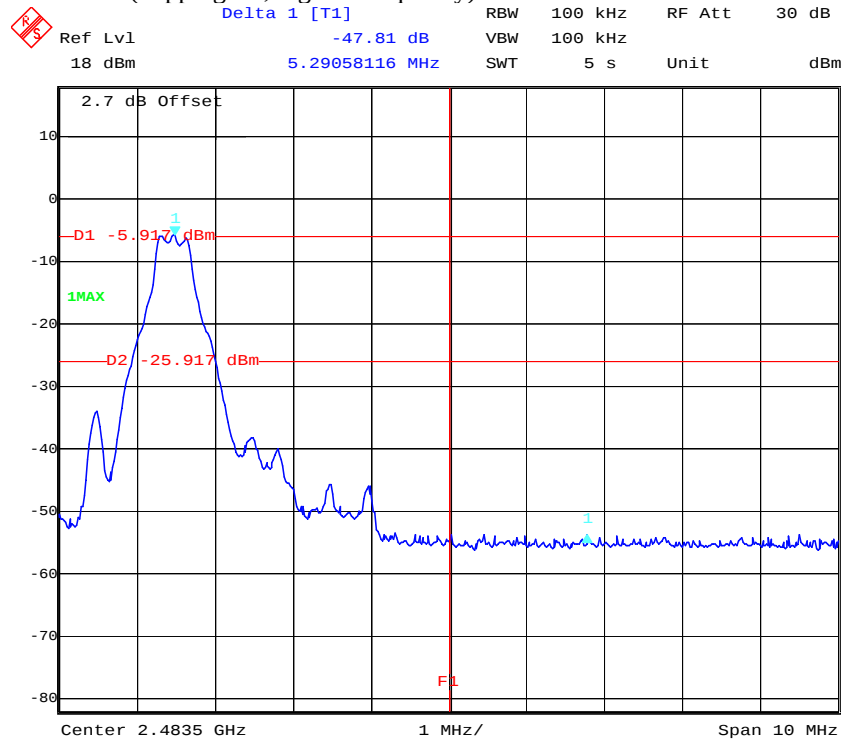
Plot 1 of 4 (hopping off, highest frequency):
