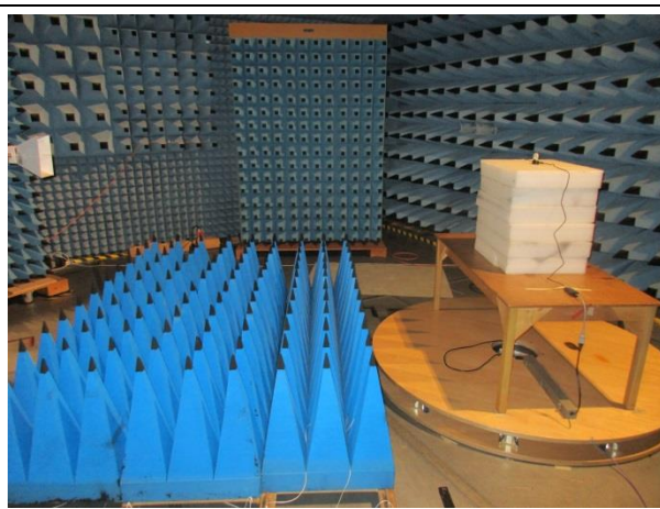
Fig 2 Radiated measurements – carrier and band edge
