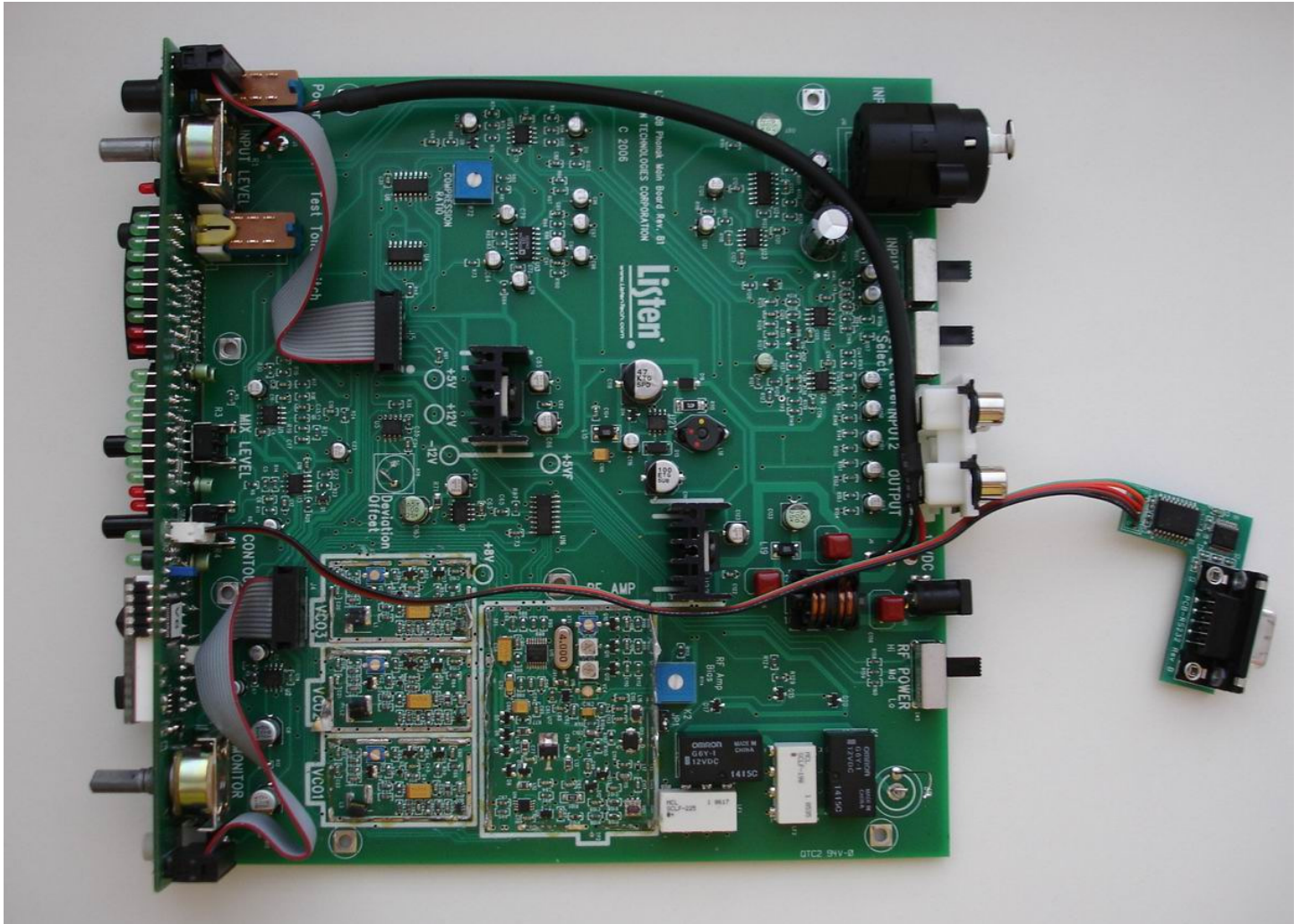
TX 300 V: Internal Photos
