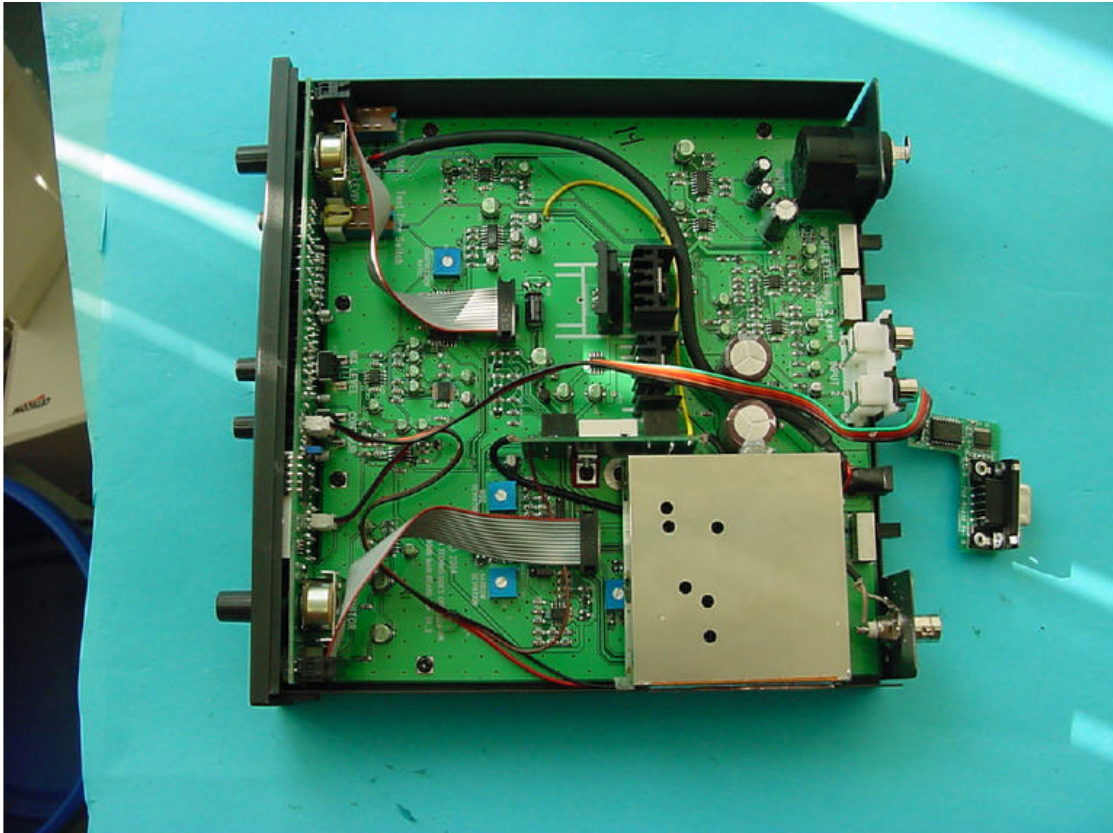
TX 300 V: Internal Photos
