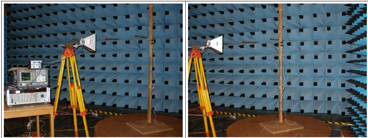
Fig 6 Radiated measurements - carrier
