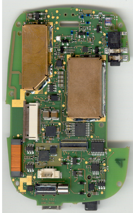
Fig 2 Phonak inspiro PCB bottom view
