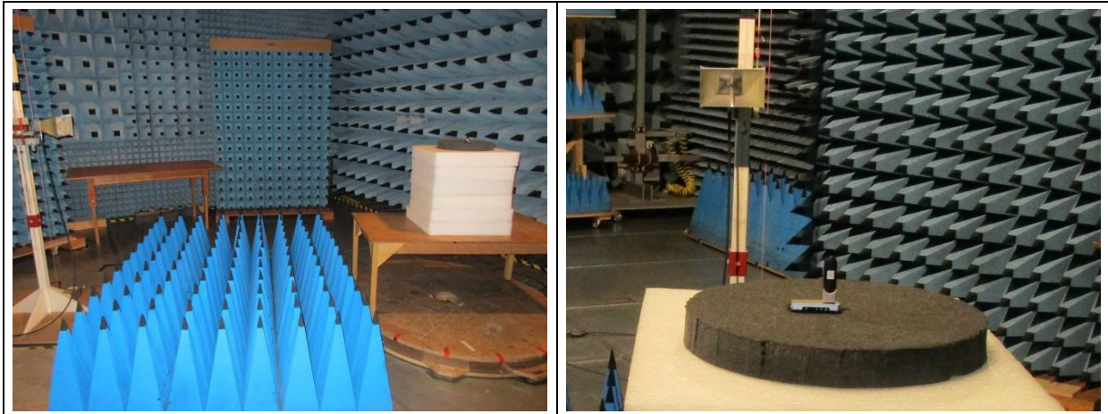
Fig 1 Radiated measurements - carrier
