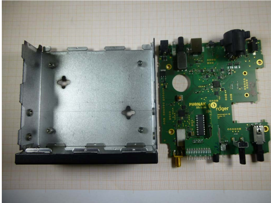
Photo 3: EUT opened
