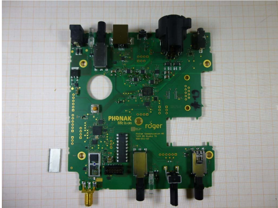
Photo 7: PCB top view without shielding
