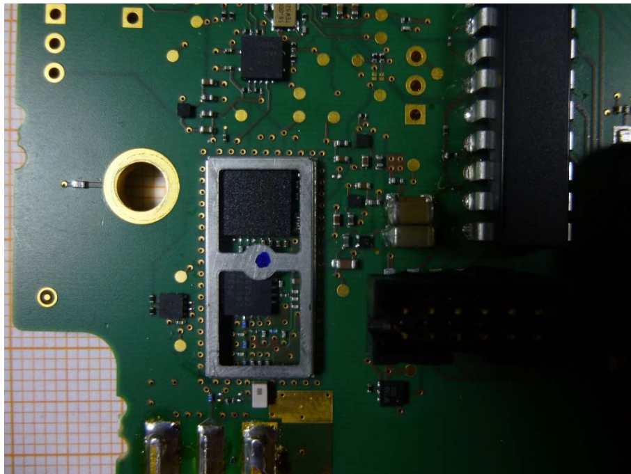
Photo 8: RF module without shielding
