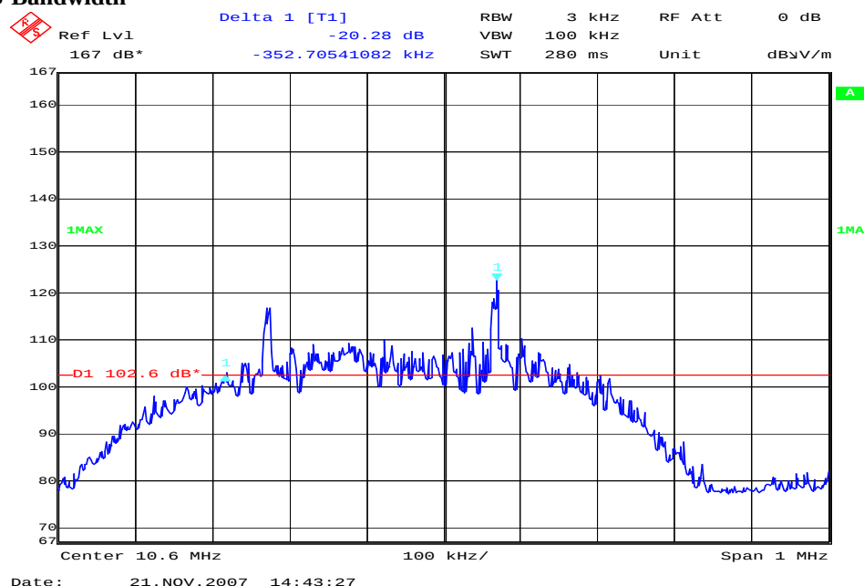
Plot 1: 20 dB-Bandwidth
