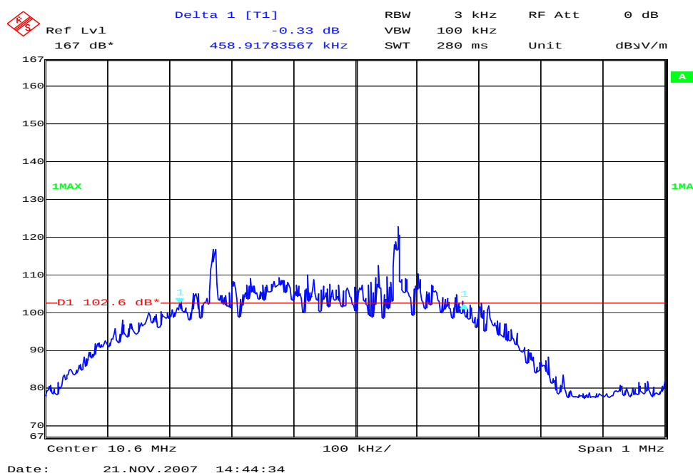
Plot 3 20 dB-Bandwidth
