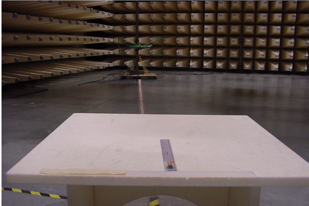
Photo 4 (Radiated Emissions):
