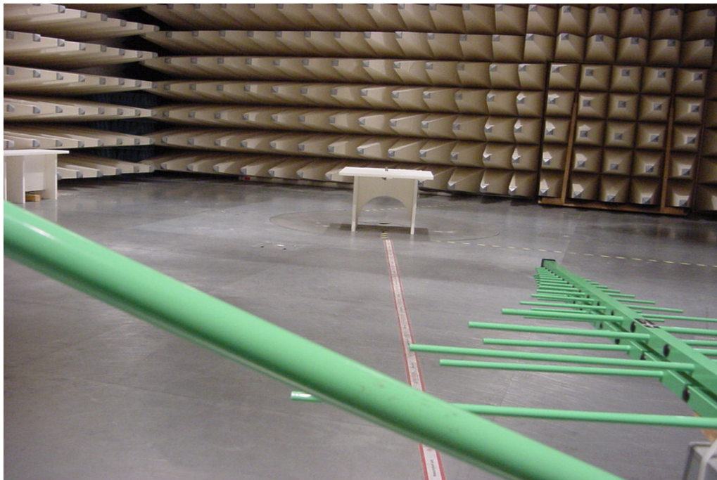
Photo 4 (Radiated Emissions):
