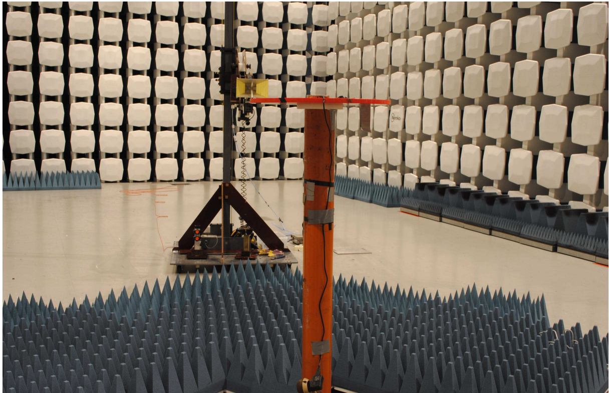
Radiated Emissions, above 1 GHz
