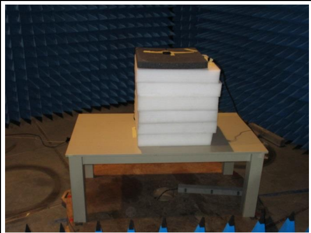
Fig 2 Radiated measurements – Carrier EIRP
