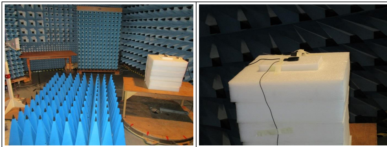
Fig 6 Radiated emission – Band edge
