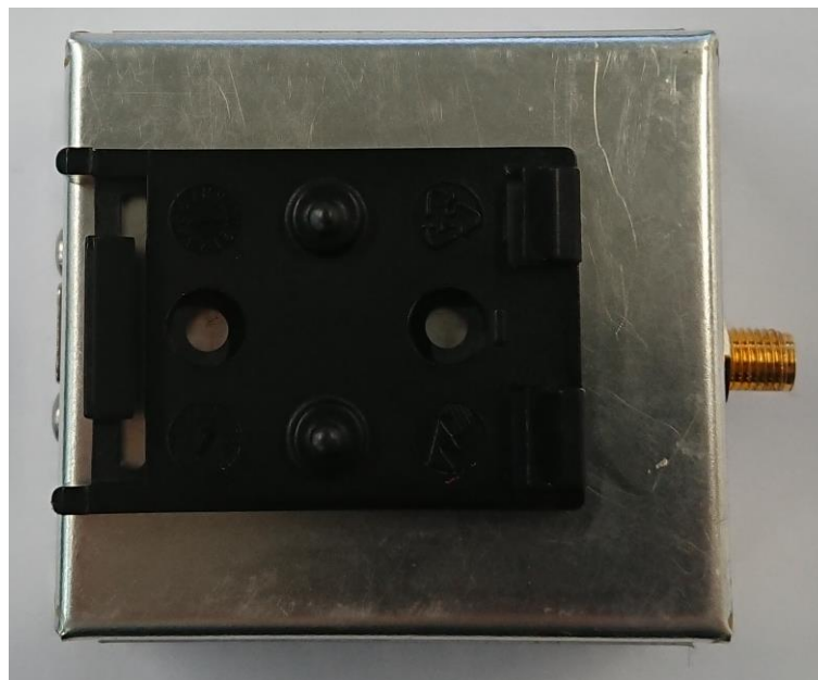
Figure 6 Excalibur bottom
