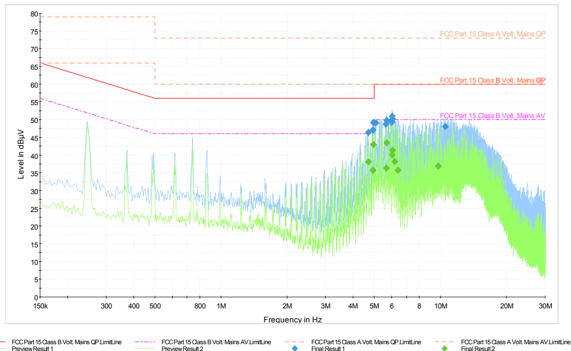
Figure 6-8: Conducted Emission Test AC Power Port (tone on)
