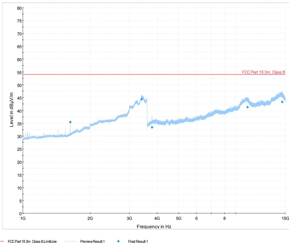
Figure 6-5: Radiated emission, 1 GHz – 15 GHz
