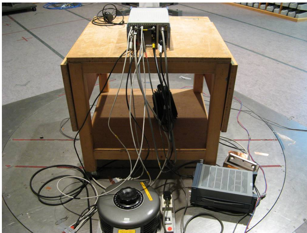
Figure 6-6: Test set-up for conducted emission measurement on the AC power port
