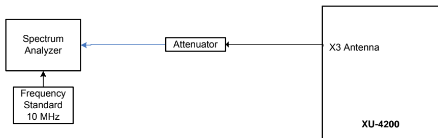
Figure 4-5: : Measurement Test Configuration
