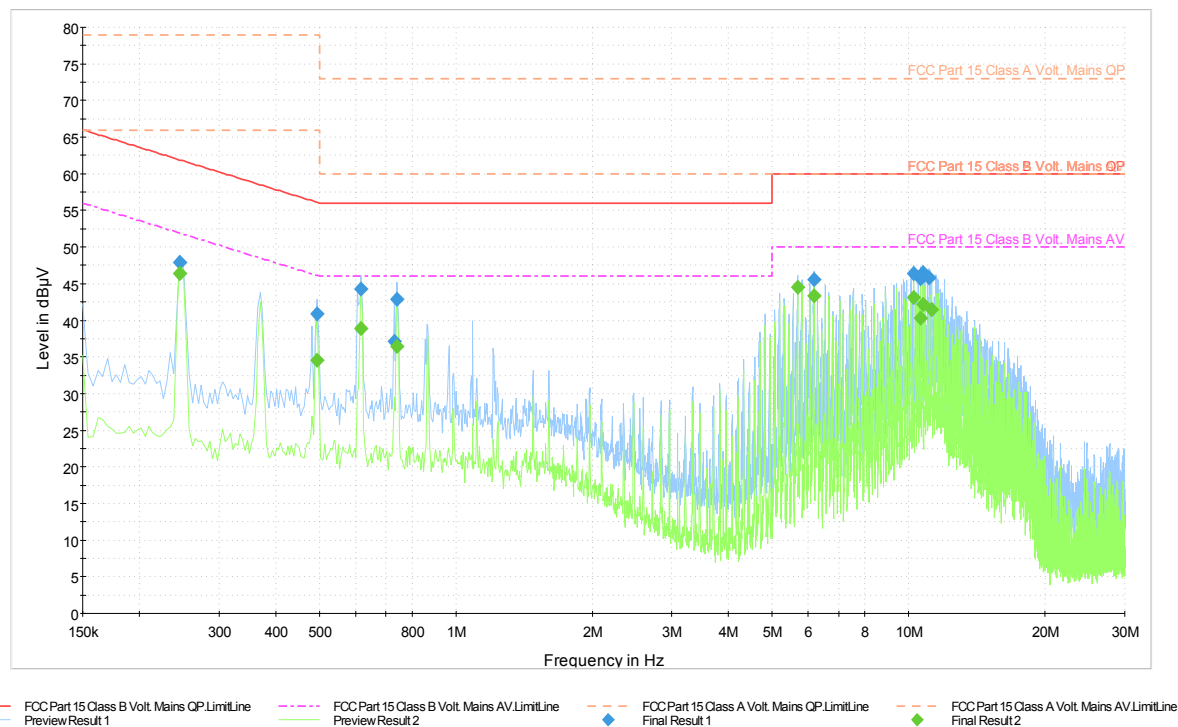
Figure 6-7: Conducted Emission Test AC Power Port (tone off)
