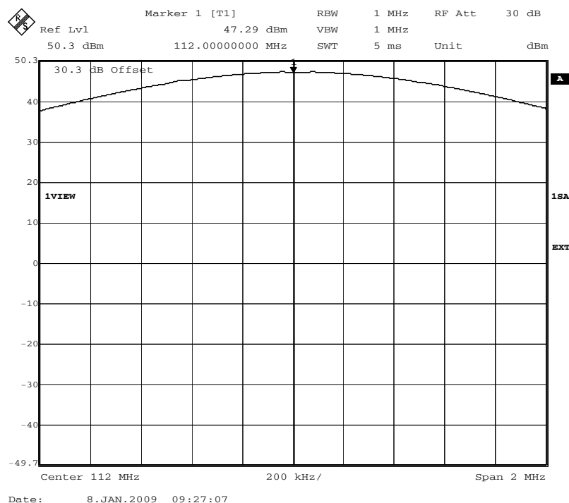
Fig. 1 –Output Power at the Antenna Connector (112.0 MHz)
