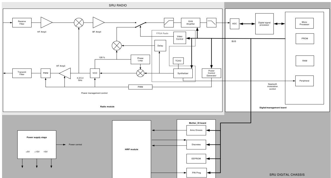
Figure 6 – General architecture of the AHV1600
