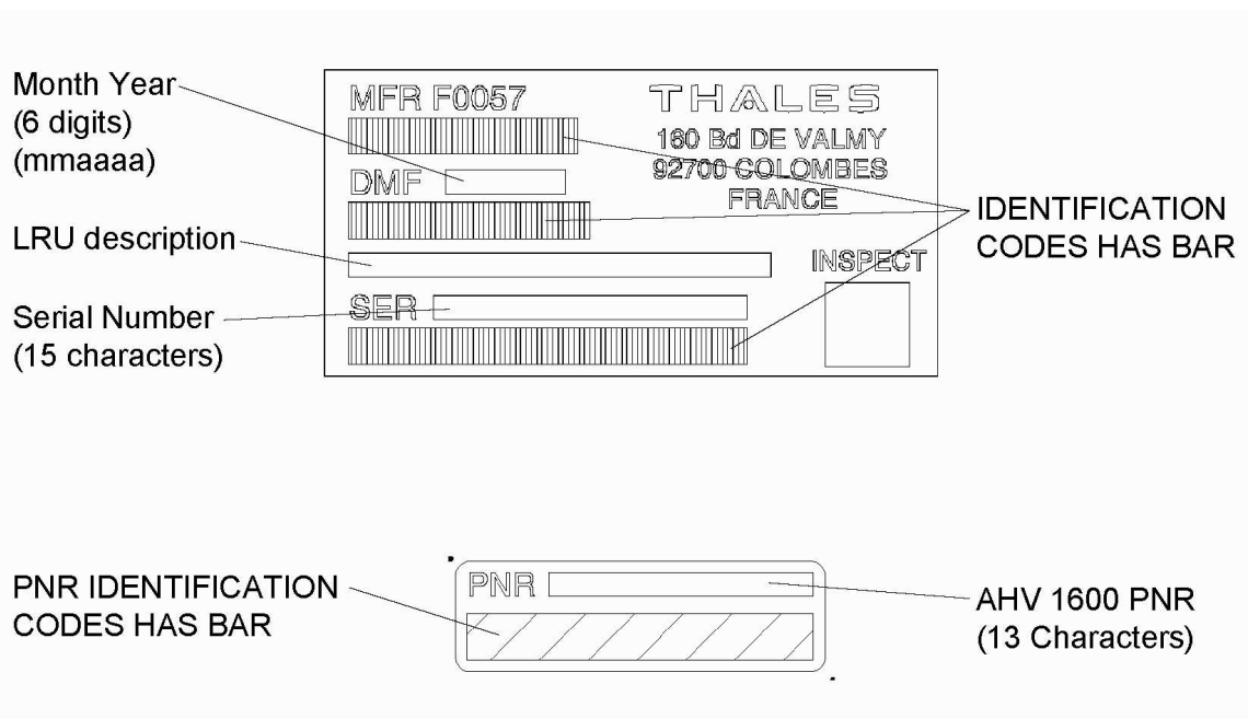
Figure 4 – Identification labels
