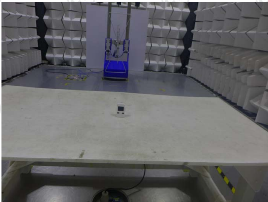
Radiated emission Test Setup-1 for WB-660(30MHz~1GHz)
