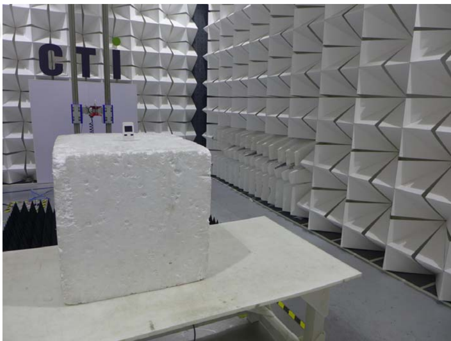
Radiated spurious emission Test Setup-4 for WB-630(Above 1GHz)
