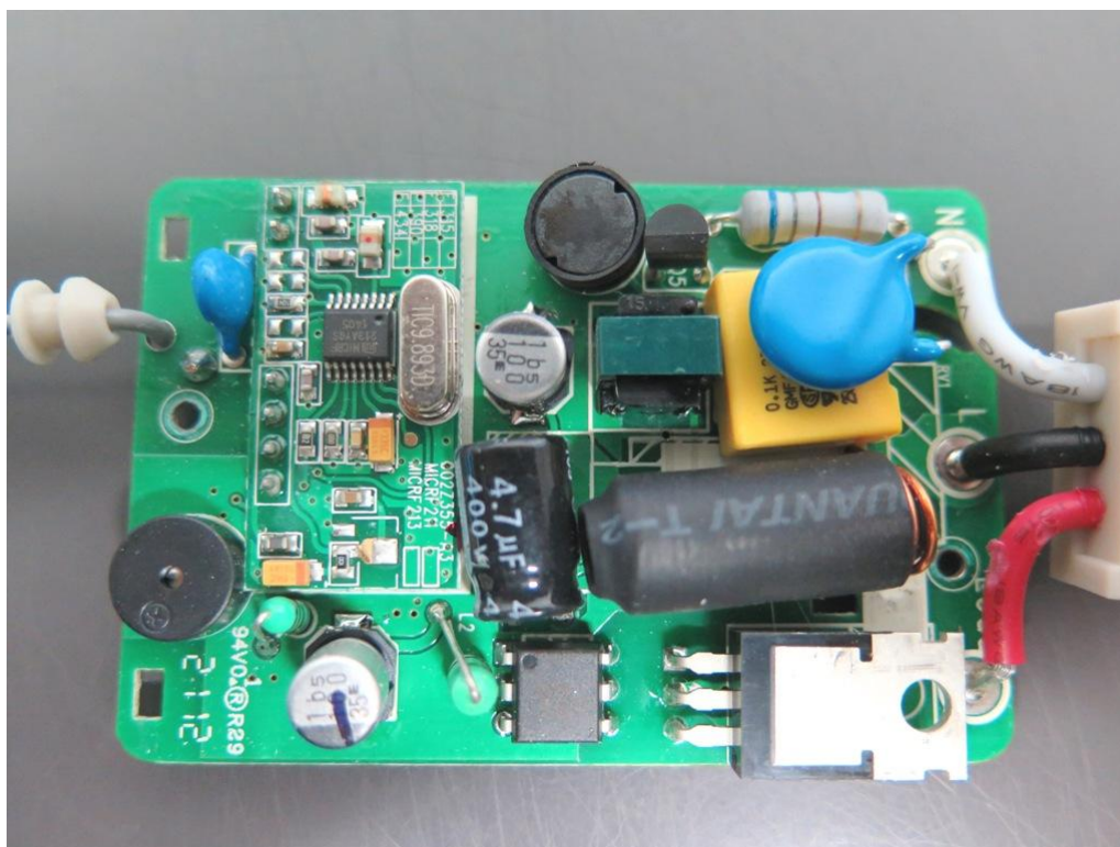
Main board
