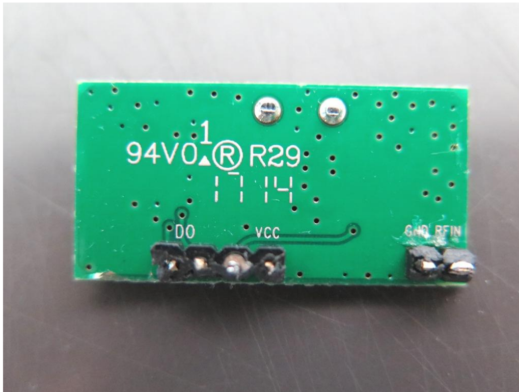
Receiver module
