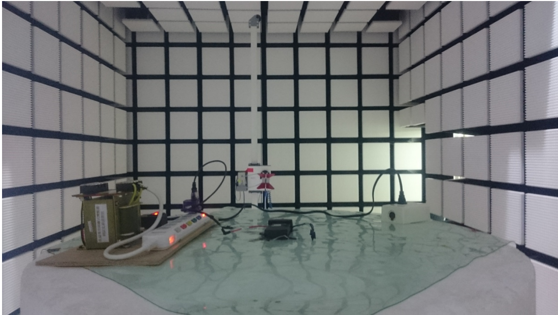
EUT with 290-80076 Second Source Antenna
