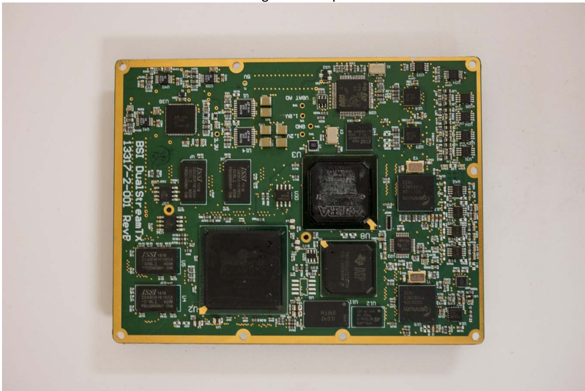
Digital PCB Top
