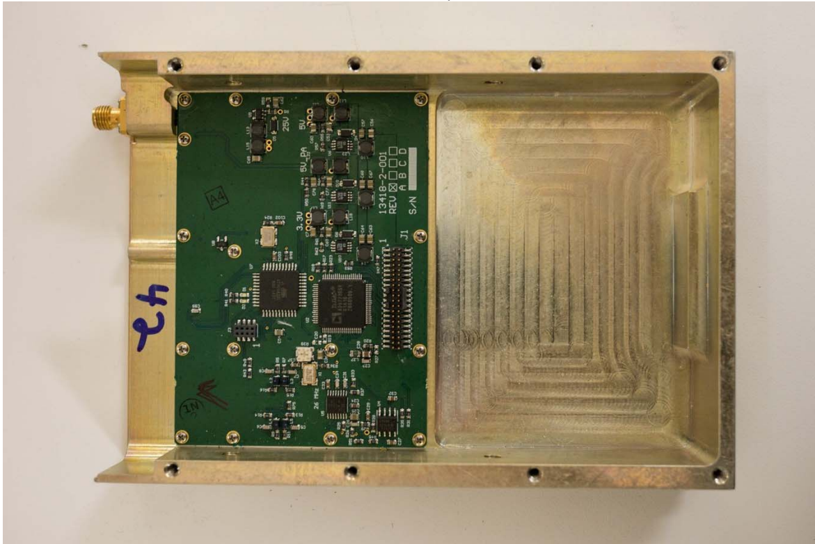
RF PCB Top
