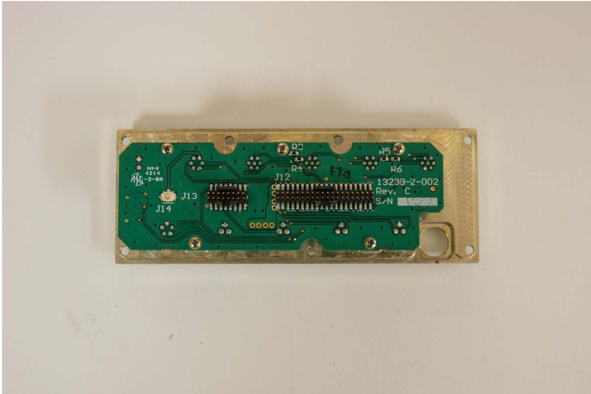
Front Panel PCB Bottom
