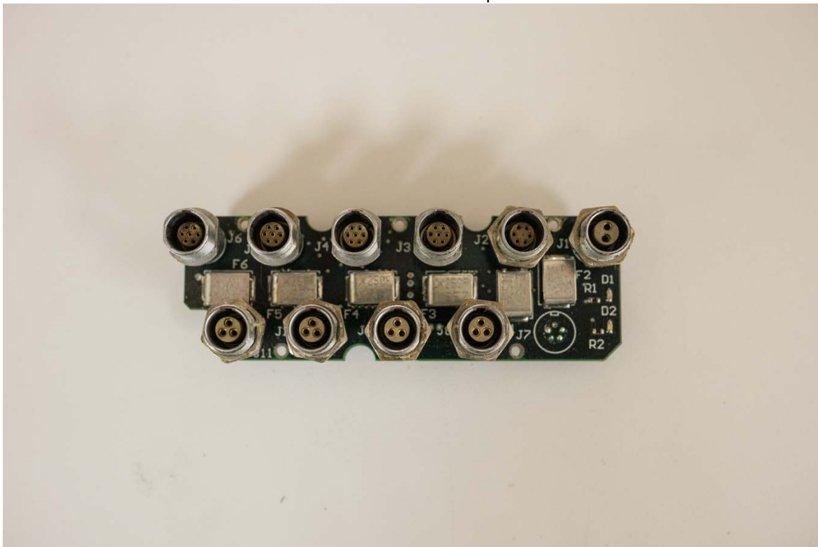
Front Panel PCB Top
