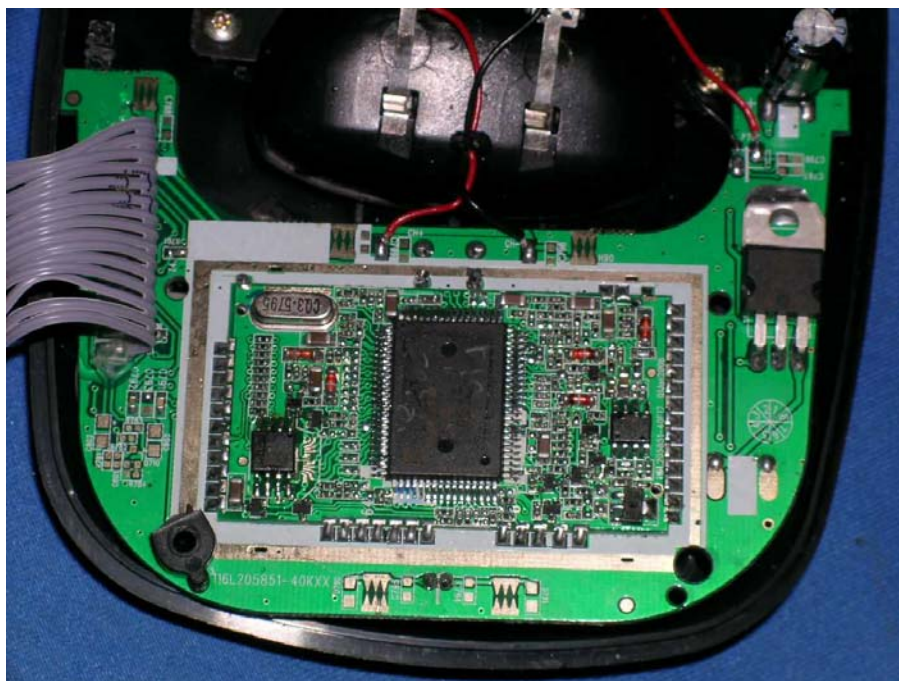
Base unit DAM rear side (View 1)
