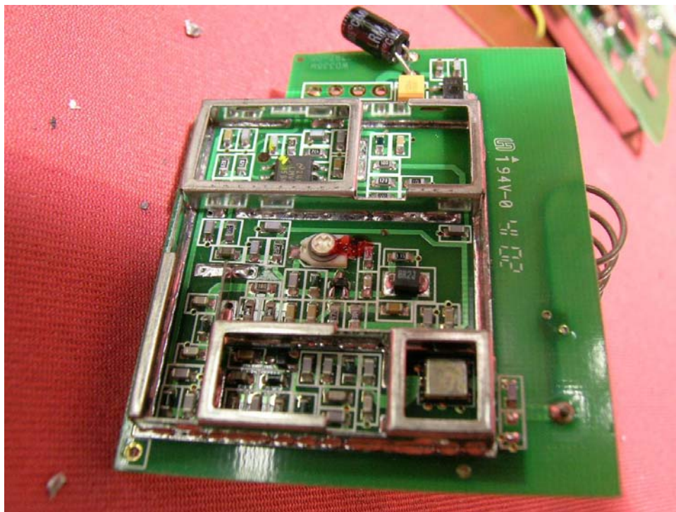
Base another Oscillator PCB comp side (View 2)
