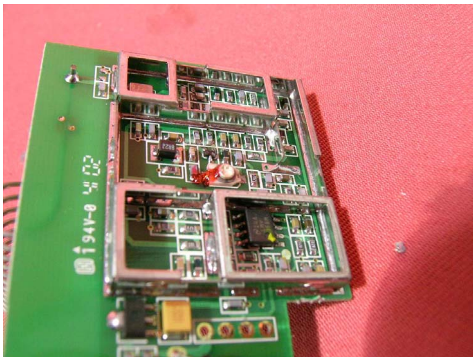
Base another Oscillator PCB comp side (View 3)
