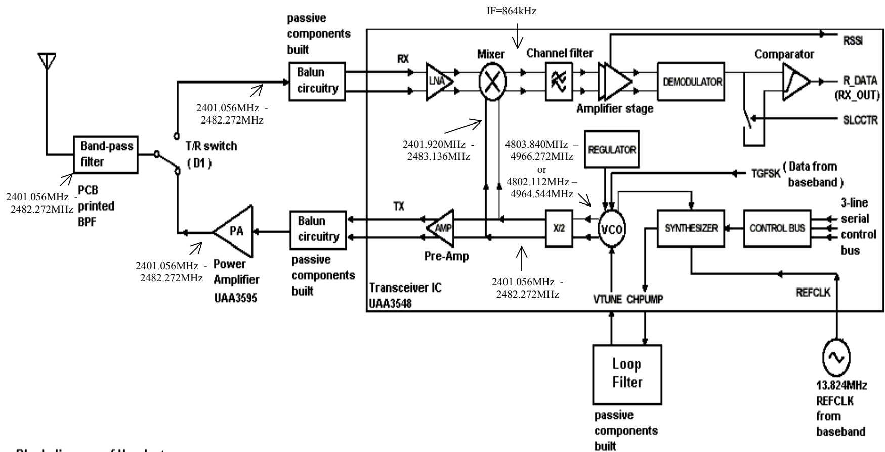
Block diagram of Handset
