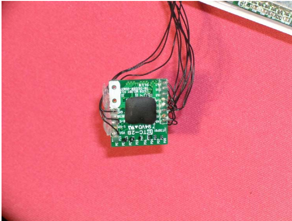
Handset Other PCB Board rear side
