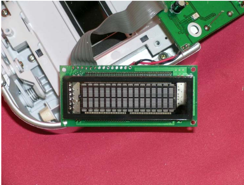
Base Display solder side
