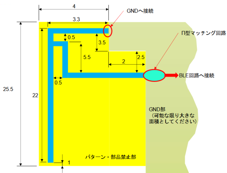
Antenna Dimension
