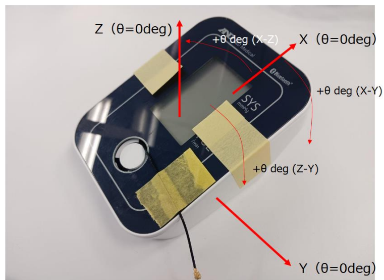
Definition of antenna measurement axis
