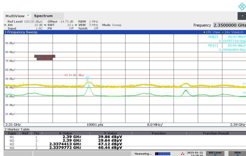
Figure 35: Restricted-band Band-edge, Spectral Diagram, Vertical Antenna Orientation, BLE, Mode L (2402MHz), 2Mbps
