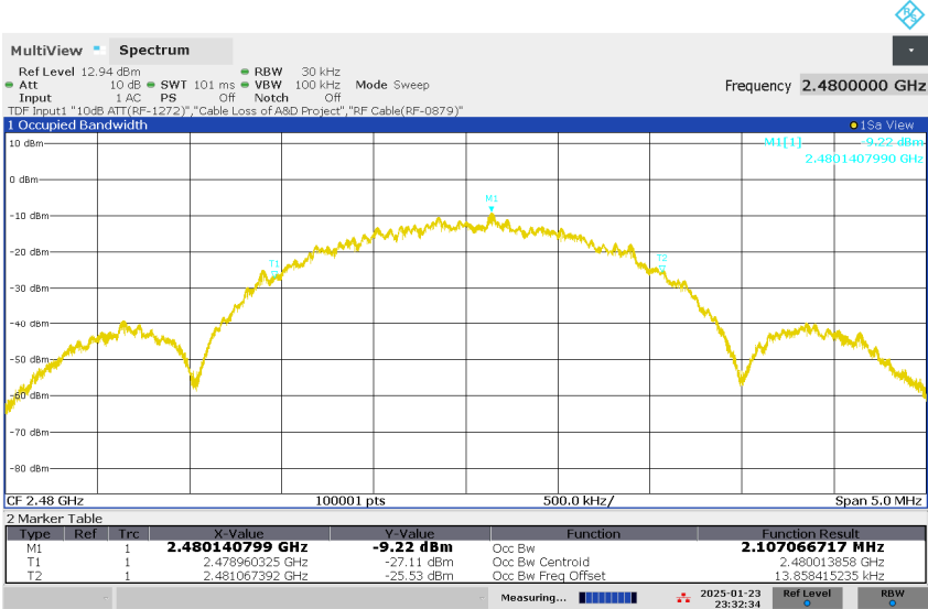
Figure 13: 99% Bandwidth, BLE, Mode H (2480MHz), 2Mbps
