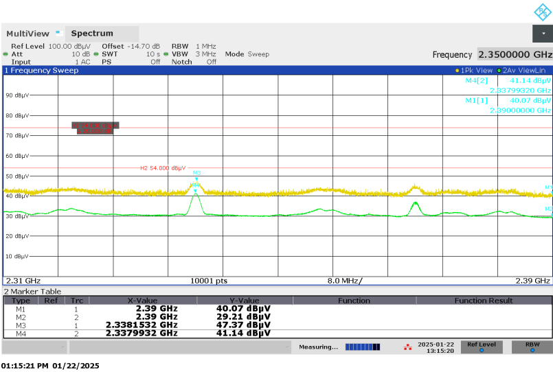
Figure 31: Restricted-band Band-edge, Spectral Diagram, Vertical Antenna Orientation, BLE, Mode L (2402MHz), 1Mbps
