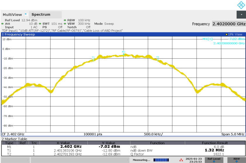
Figure 5: 6dB Bandwidth, BLE, Mode L (2402MHz), 2Mbps
