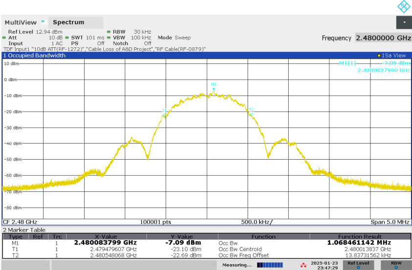
Figure 10: 99% Bandwidth, BLE, Mode H (2480MHz), 1Mbps
