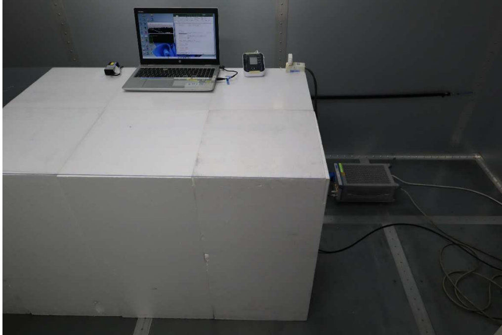
Photograph 8: Set-up for AC Power Line Conducted Emission, Front View
