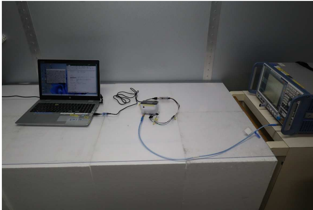
Photograph 1: Set-up for Antenna Port Conducted Emission of Transmitter, General View
