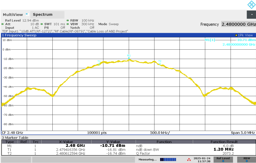
Figure 7: 6dB Bandwidth, BLE, Mode H (2480MHz), 2Mbps
