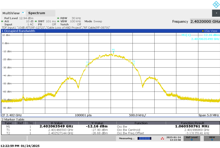
Figure 8: 99% Bandwidth, BLE, Mode L (2402MHz), 1Mbps
