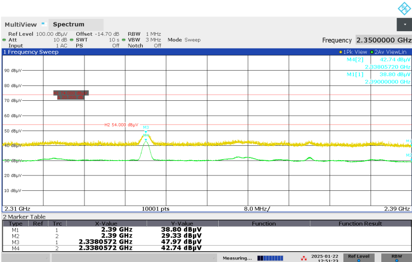
Figure 30: Restricted-band Band-edge, Spectral Diagram, Horizontal Antenna Orientation, BLE, Mode L (2402MHz), 1Mbps
