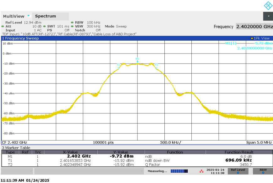
Figure 2: 6dB Bandwidth, BLE, Mode L (2402MHz), 1Mbps
