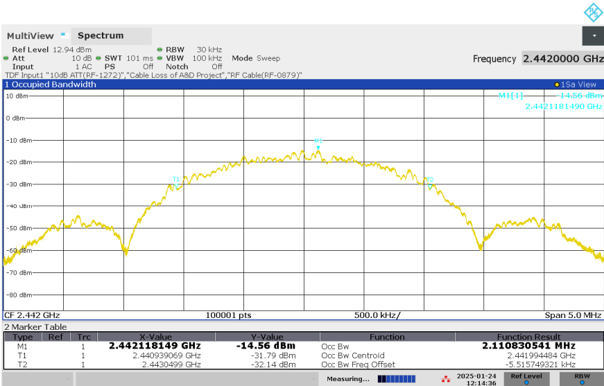
Figure 12: 99% Bandwidth, BLE, Mode M (2442MHz), 2Mbps
