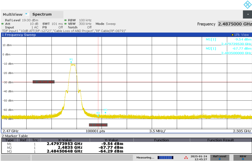
Figure 18: Authorized-band band-edge, BLE, Mode H (2480MHz), 1Mbps
