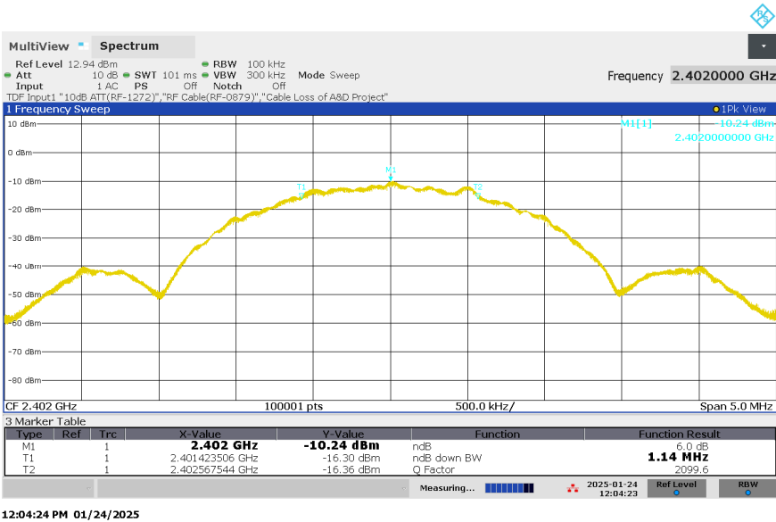
Figure 5: 6dB Bandwidth, BLE, Mode L (2402MHz), 2Mbps
