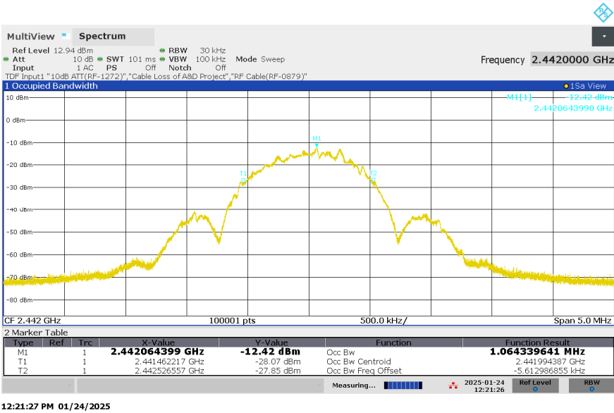
Figure 9: 99% Bandwidth, BLE, Mode M (2442MHz), 1Mbps
