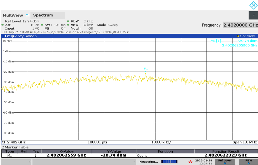
Figure 24: Power Spectral Density, BLE, Mode L (2402MHz), 1Mbps
