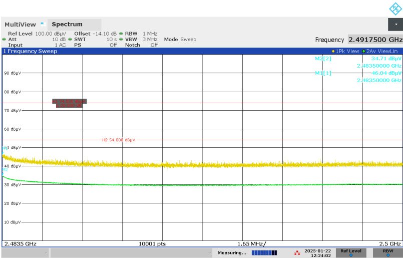
Figure 36: Restricted-band Band-edge, Spectral Diagram, Horizontal Antenna Orientation, BLE, Mode H (2480MHz), 2Mbps
