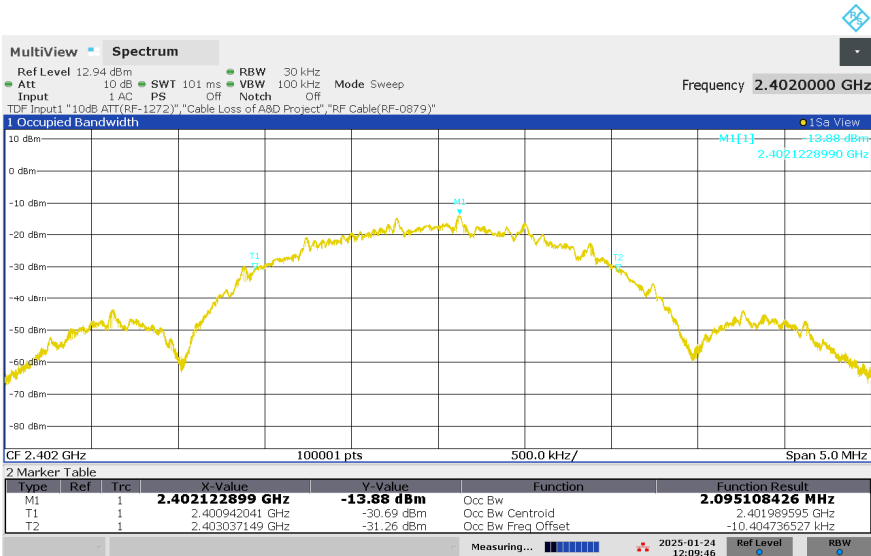
Figure 11: 99% Bandwidth, BLE, Mode L (2402MHz), 2Mbps
