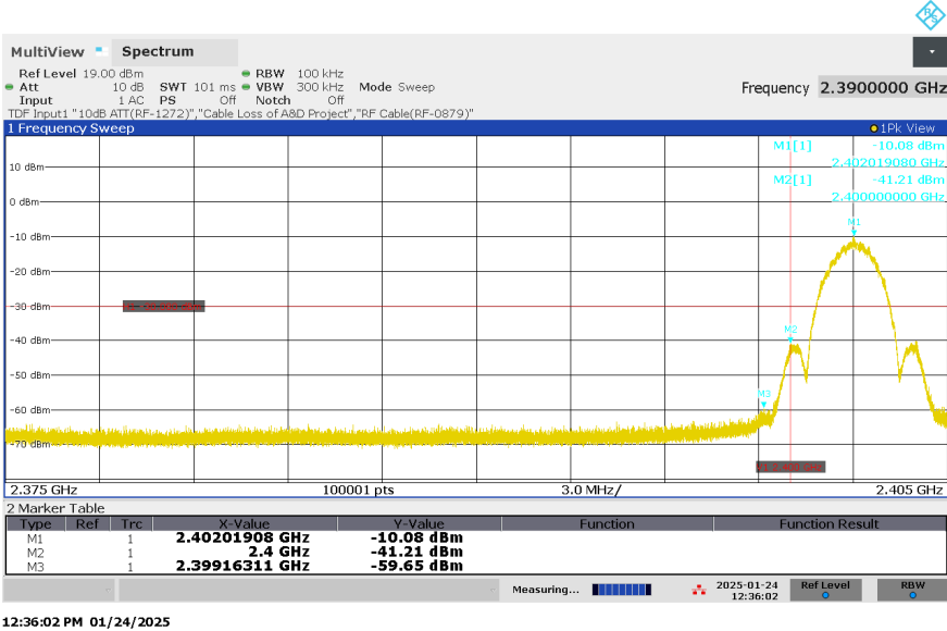
Figure 22: Authorized-band band-edge, BLE, Mode L (2402MHz), 2Mbps
