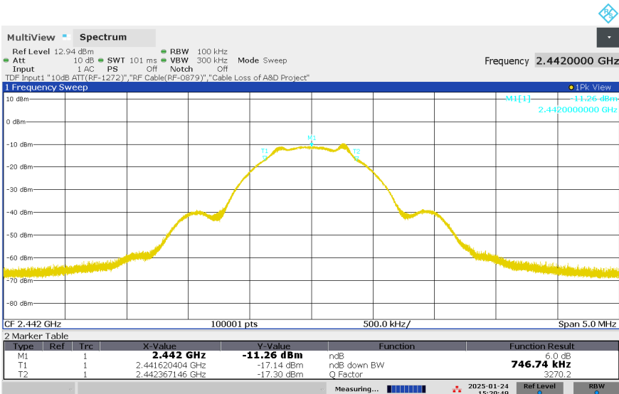
Figure 3: 6dB Bandwidth, BLE, Mode M (2442MHz), 1Mbps
