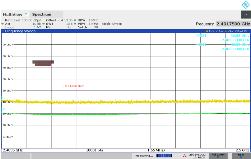
Figure 32: Restricted-band Band-edge, Spectral Diagram, Horizontal Antenna Orientation, BLE, Mode H (2480MHz), 1Mbps
