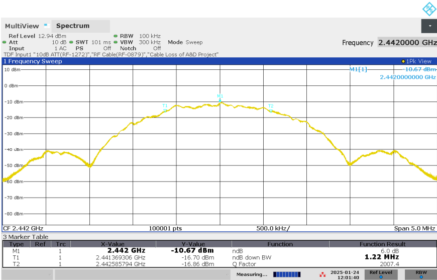
Figure 6: 6dB Bandwidth, BLE, Mode M (2442MHz), 2Mbps
