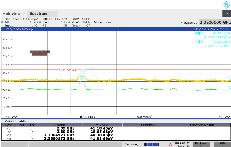
Figure 34: Restricted-band Band-edge, Spectral Diagram, Horizontal Antenna Orientation, BLE, Mode L (2402MHz), 2Mbps
