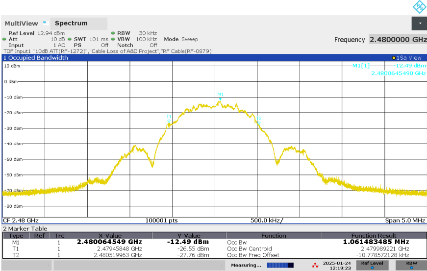
Figure 10: 99% Bandwidth, BLE, Mode H (2480MHz), 1Mbps
