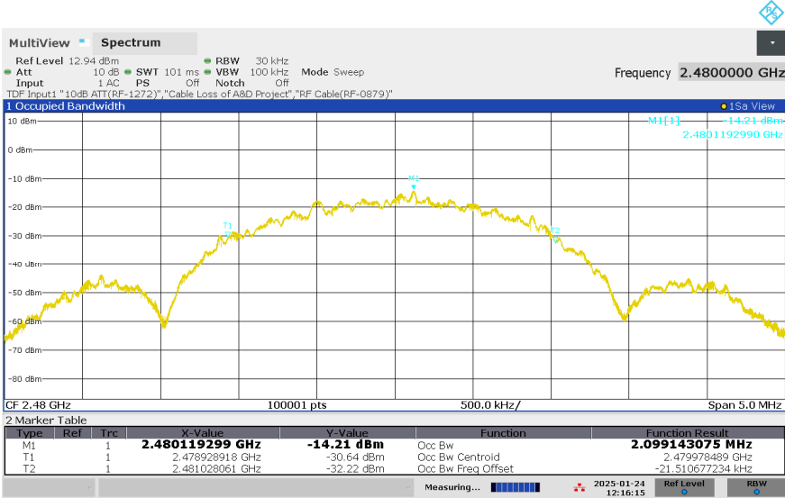
Figure 13: 99% Bandwidth, BLE, Mode H (2480MHz), 2Mbps
