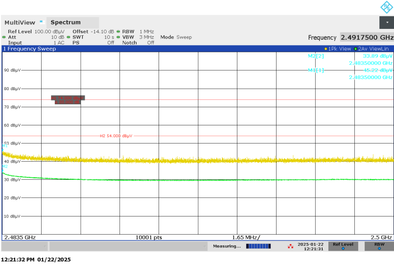
Figure 37: Restricted-band Band-edge, Spectral Diagram, Vertical Antenna Orientation, BLE, Mode H (2480MHz), 2Mbps
