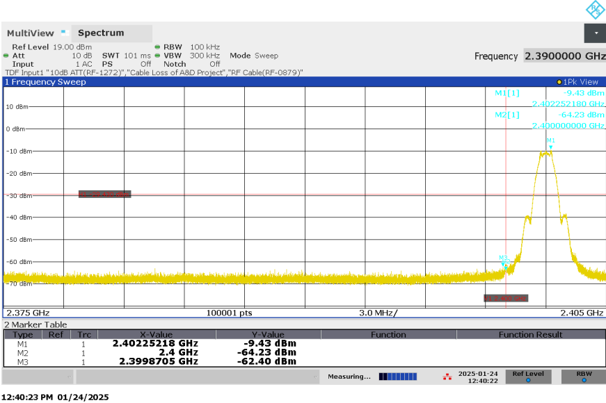
Figure 17: Authorized-band band-edge, BLE, Mode L (2402MHz), 1Mbps
