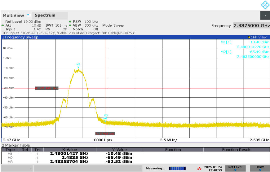
Figure 23: Authorized-band band-edge, BLE, Mode H (2480MHz), 2Mbps
