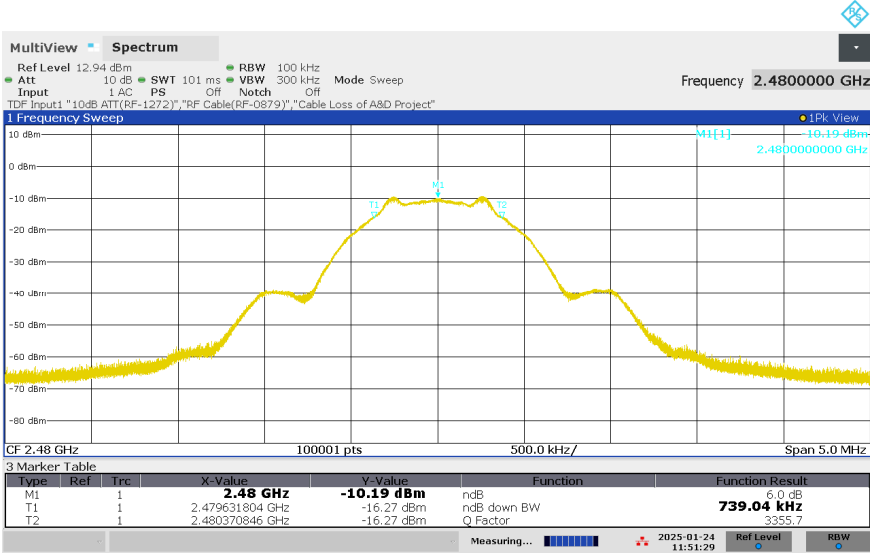
Figure 4: 6dB Bandwidth, BLE, Mode H (2480MHz), 1Mbps
