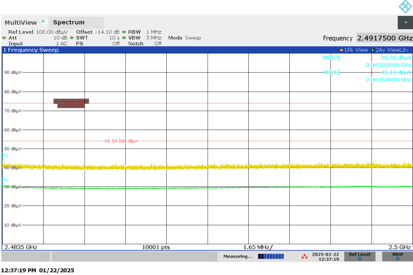
Figure 33: Restricted-band Band-edge, Spectral Diagram, Vertical Antenna Orientation, BLE, Mode H (2480MHz), 1Mbps
