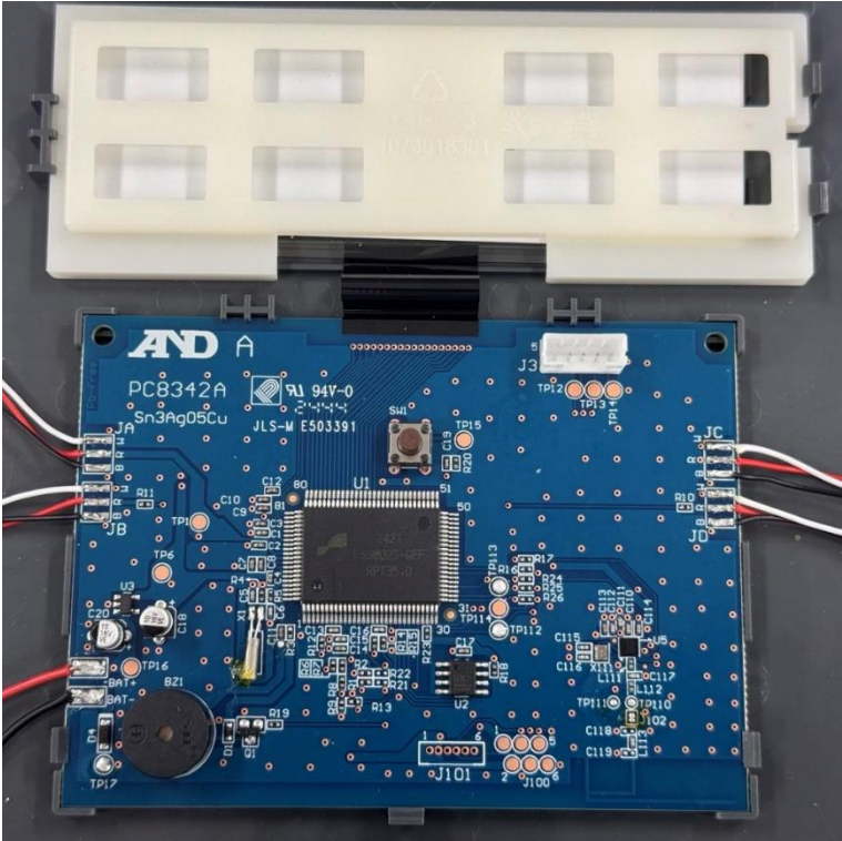
LCD and Board
