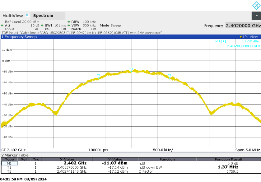
Figure 5: 6dB Bandwidth, BLE, Mode L (2402MHz), 2Mbps
