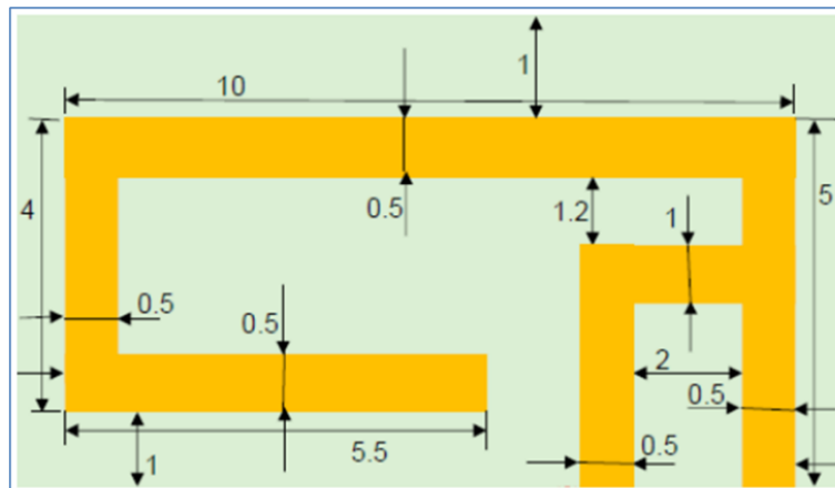
Antenna Dimension
