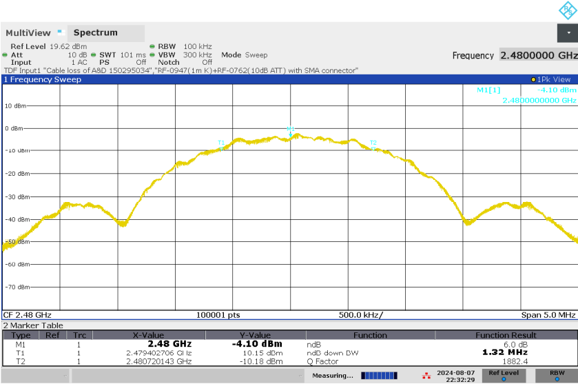
Figure 7: 6dB Bandwidth, BLE, Mode H (2480MHz), 2Mbps
