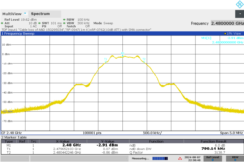
Figure 4: 6dB Bandwidth, BLE, Mode H (2480MHz), 1Mbps
