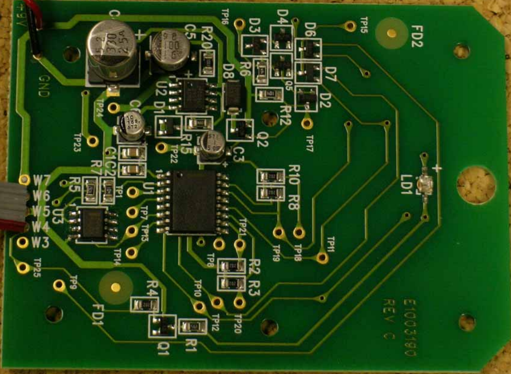
PCB (bottom)
